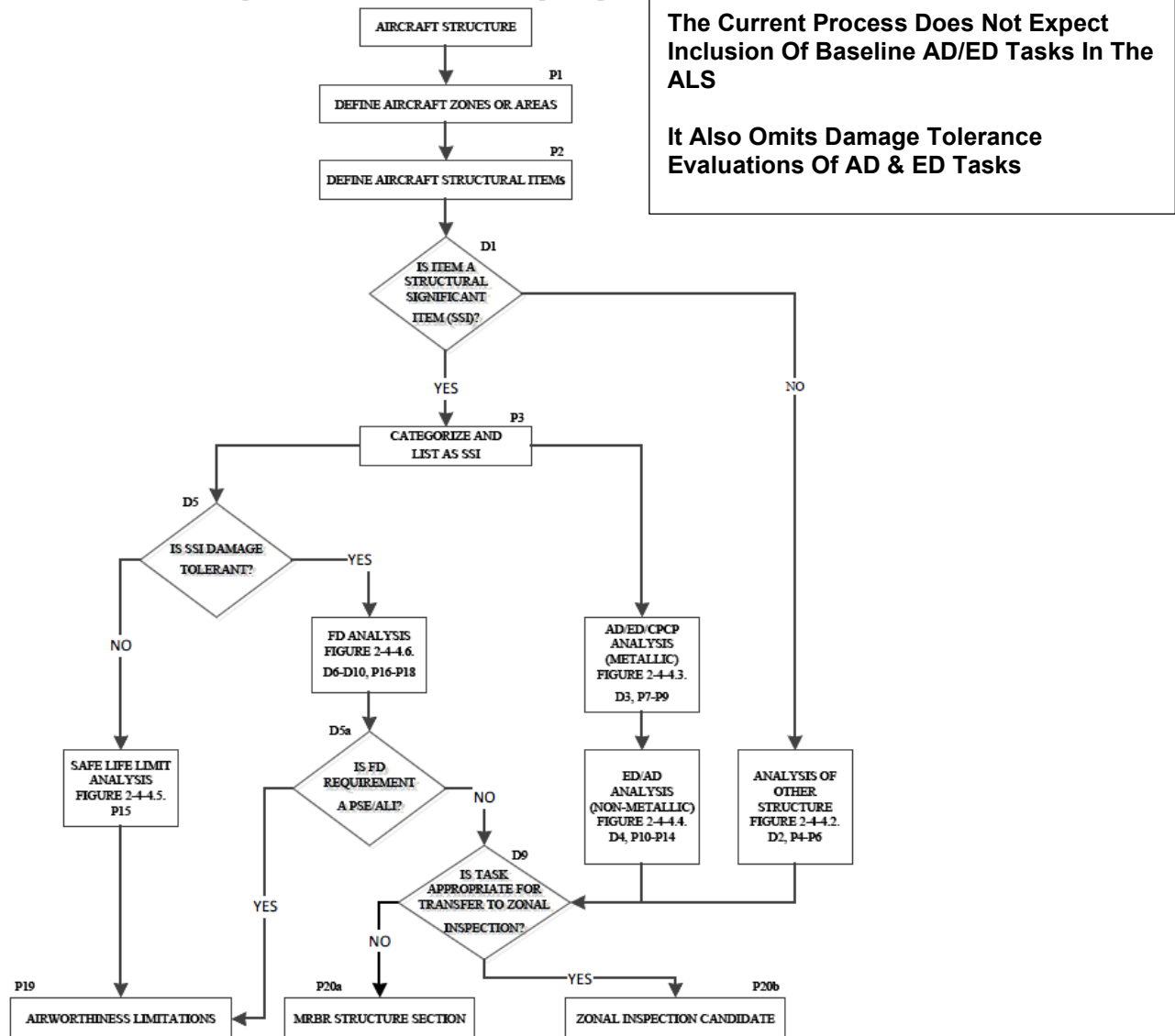
Figure 2-4-4.1. Structure MSG-3 Logic Diagram
