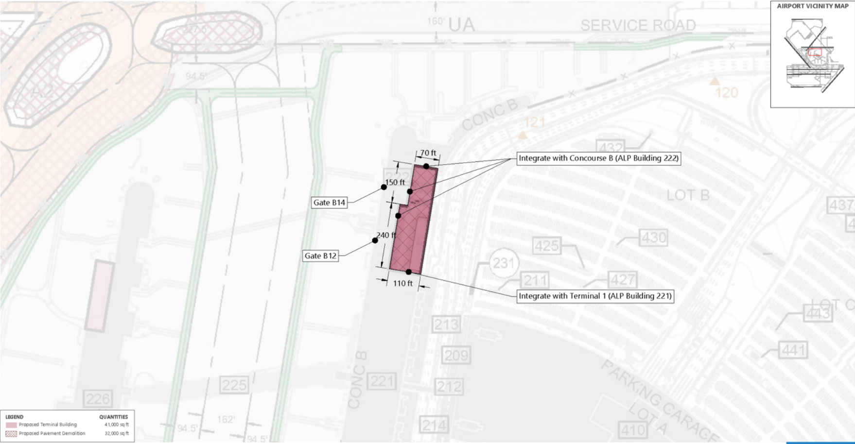
Proposed Terminal 1 Concourse B Northeast End Expansion
