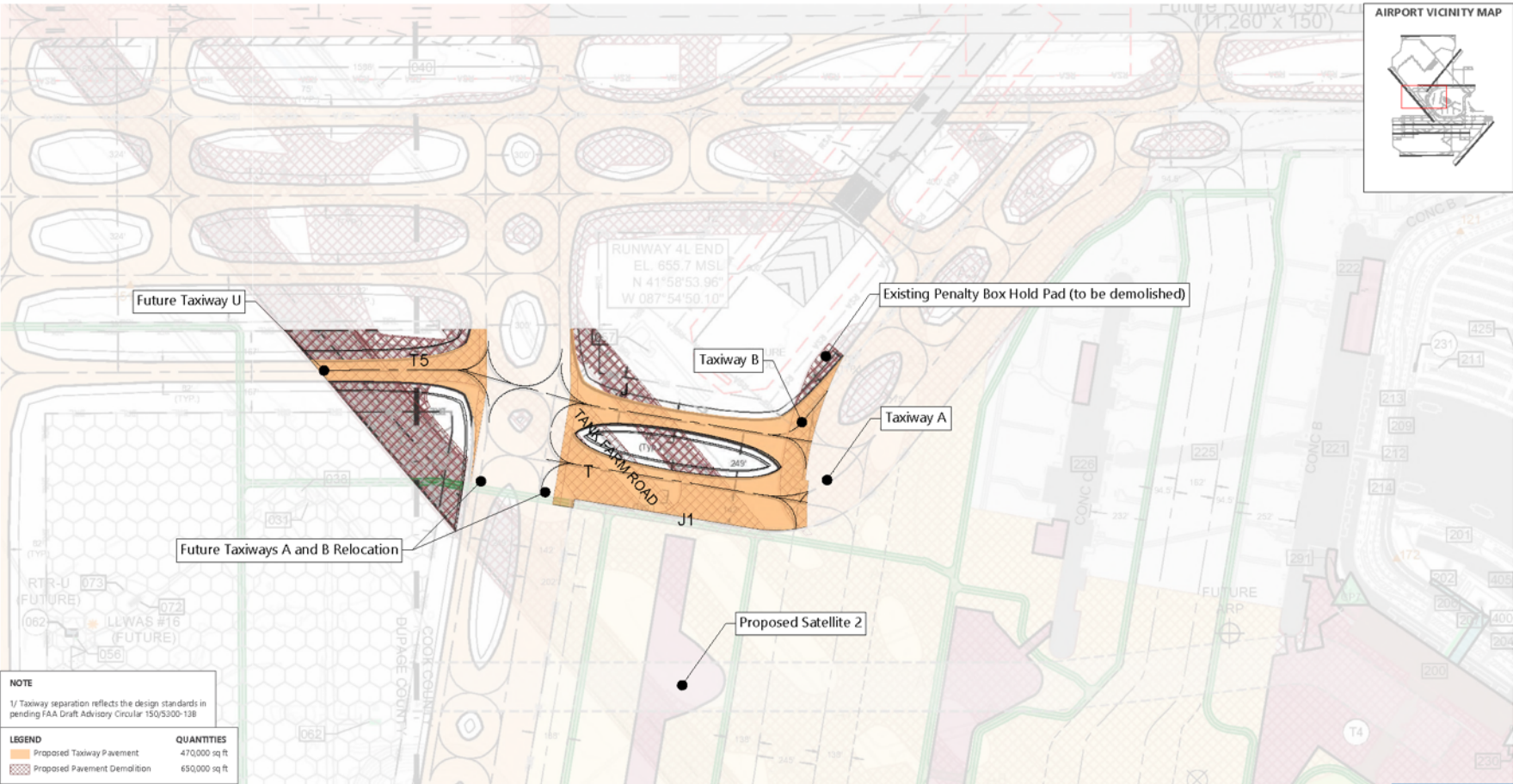
Proposed Taxiways North of Satellite 2
