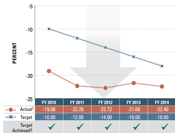
National Airspace System Energy Efficiency Cumulative percentage reduction from baseline
