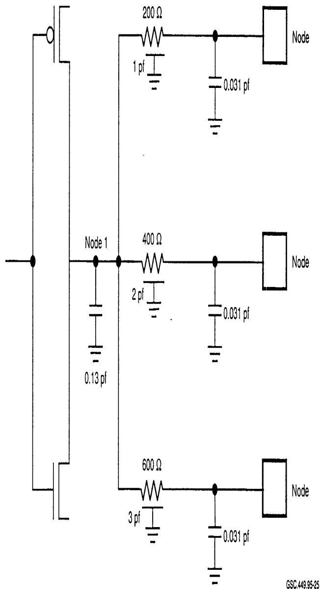
FIGURE 25. INTERCONNECT ESTIMATION FOR DEEP SUBMICRON DESIGNS (Gallant 1995)
