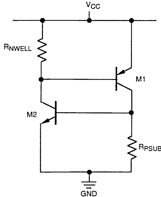
FIGURE 26. PARASITIC SILICON CONTROLLED RECTIFIER STRUCTURE
