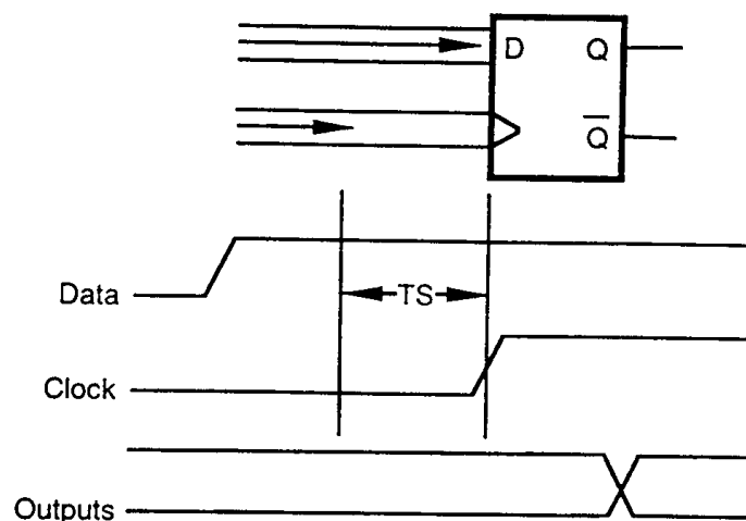
FIGURE 21. SETUP-TIME ILLUSTRATION FOR POSITIVE EDGE CLOCKED FLIP-FLOP
