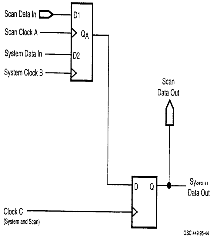
FIGURE 53. LEVEL SENSITIVE SCAN DESIGN SCAN REGISTER CONFIGURATION (Oakland et al. 1994)
