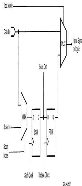
FIGURE 58. BOUNDARY SCAN TEST INPUT CELL CONF]GURATION (Pointers 1994)
