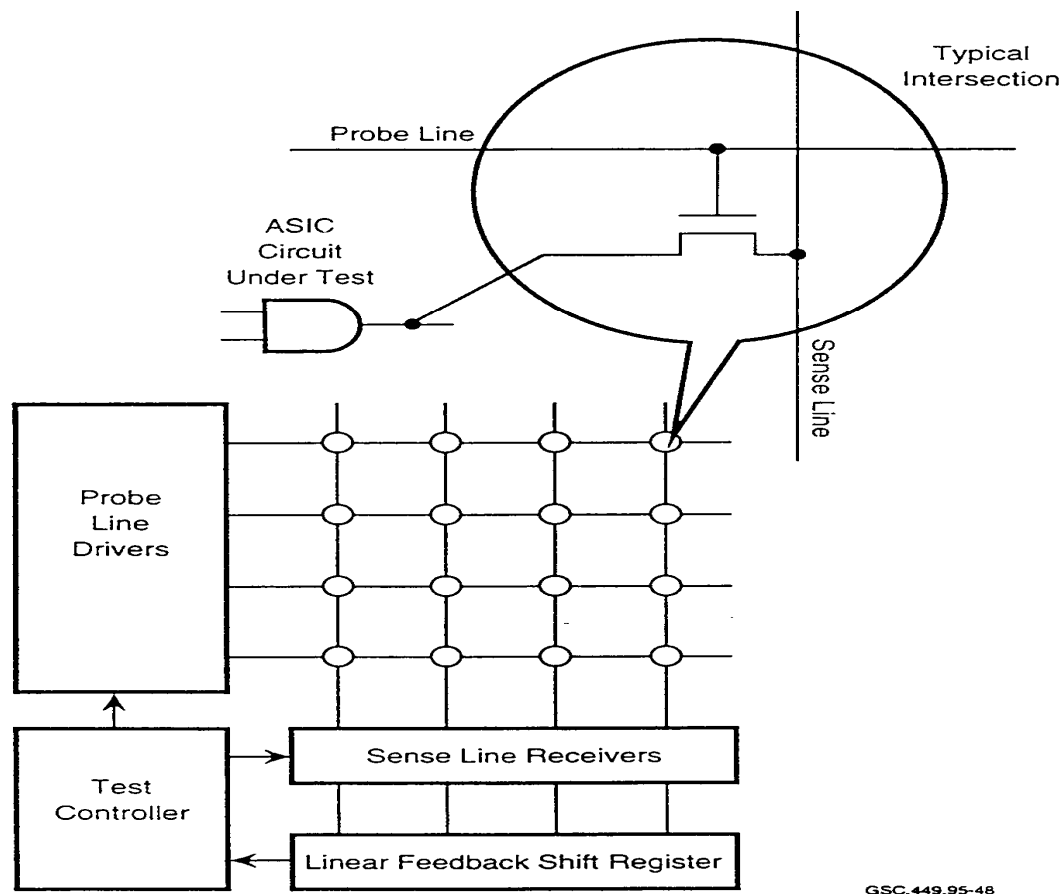
FIGURE 60 CROSSCHECK™ CONFIGURATION (Levitt 1992)
