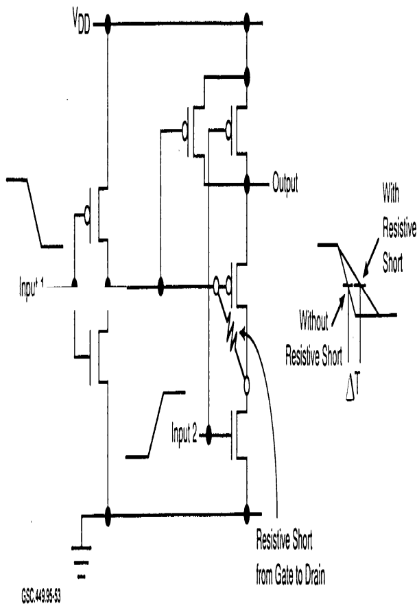
FIGURE 65. GATE TO DRAIN SHORT (Mascitelli 1994)
