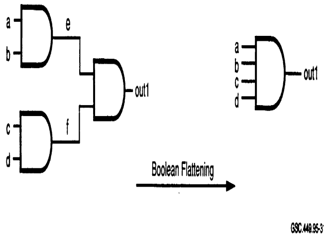
FIGURE 33b. BOOLEAN FLATTENING
