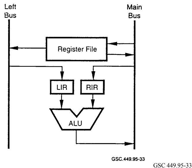
FIGURE 38. A TWO-BUS DESIGN IMPLEMENTATION USING PIPELINING
