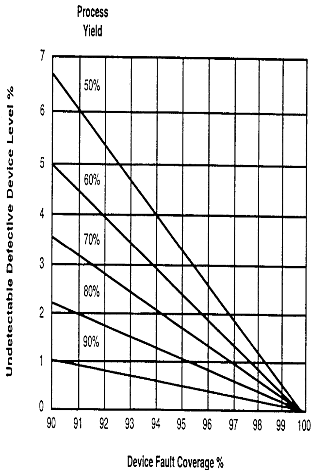
FIGURE 45. PERCENT OF UNDETECTABLE DEFECTIVE DEVICES (Gruebel 1995)
