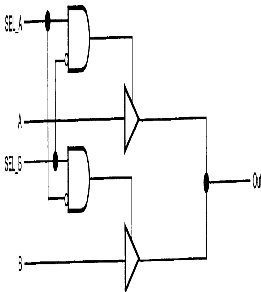
FIGURE 20. AVOIDING BUS CONTENTION BY DESIGN (Zeidman 1994)
