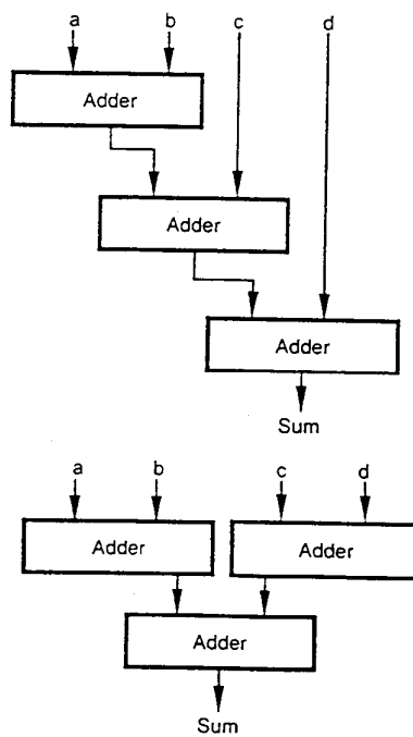
FIGURE 41. ADDER CARRY IMPLEMENTATIONS (Widman 1994)
