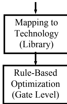
FIGURE 32. LOGIC SYNTHESIS PROCESS (Widman 1994)
