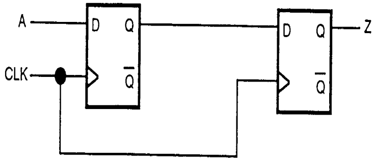
FIGURE 22. SYNCHRONIZATION OF ASYNCHRONOUS SIGNAL
