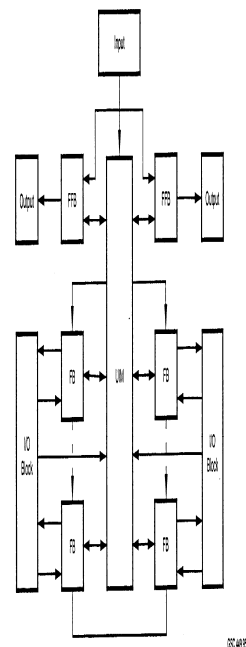
FIGURE 5. EPLD BLOCK DIAGRAM (Programmable Logic Data Book 1994)
