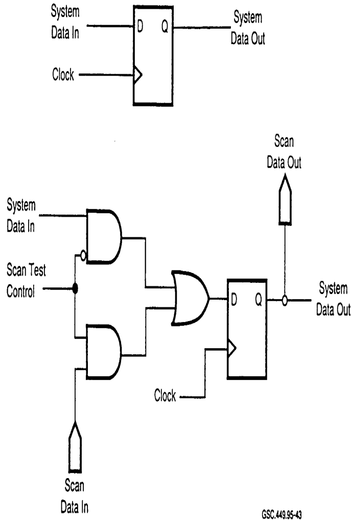
FIGURE 52. MUX-SCAN CIRCUIT CONFIGURATION (Oakland et al. 1994)
