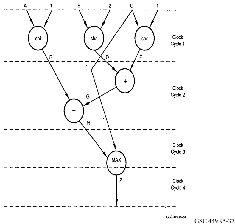
FIGURE 39. SCHEDULER EXAMPLE
