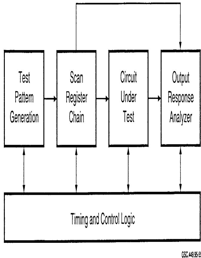
FIGURE 51. SCANBIST BLOCK DIAGRAM
