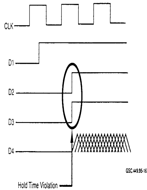
FIGURE 16. HOLD-TIME VIOLATION (Zeidman 1994)
