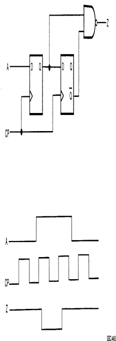
FIGURE 15. CLOCK-BASED INDEPENDENT DELAY LOGIC (Zeidman 1994)
