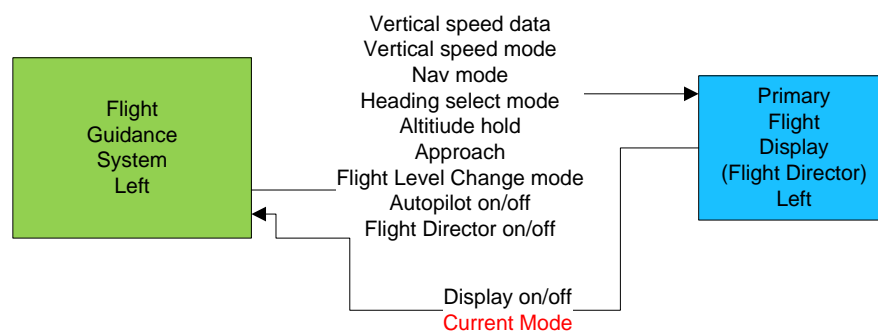
Figure B-3. FGS left interactions with PFD
