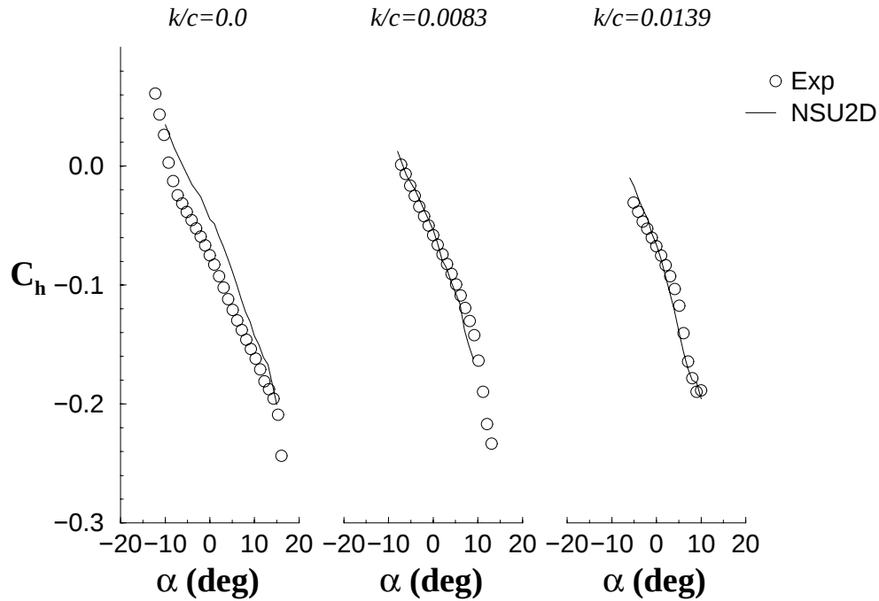
FIGURE 136. EFFECT OF ICE SHAPE HEIGHT ON HINGE MOMENT FOR A NLF 0414 AIRFOIL WITH A QUARTER-ROUND ICE SHAPE LOCATED AT x/c = 0.1
