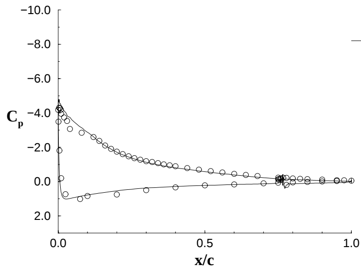
FIGURE 37. SURFACE PRESSURE DISTRIBUTION FOR A NACA 23012m AIRFOIL AT \alpha = 12.36^\circ
