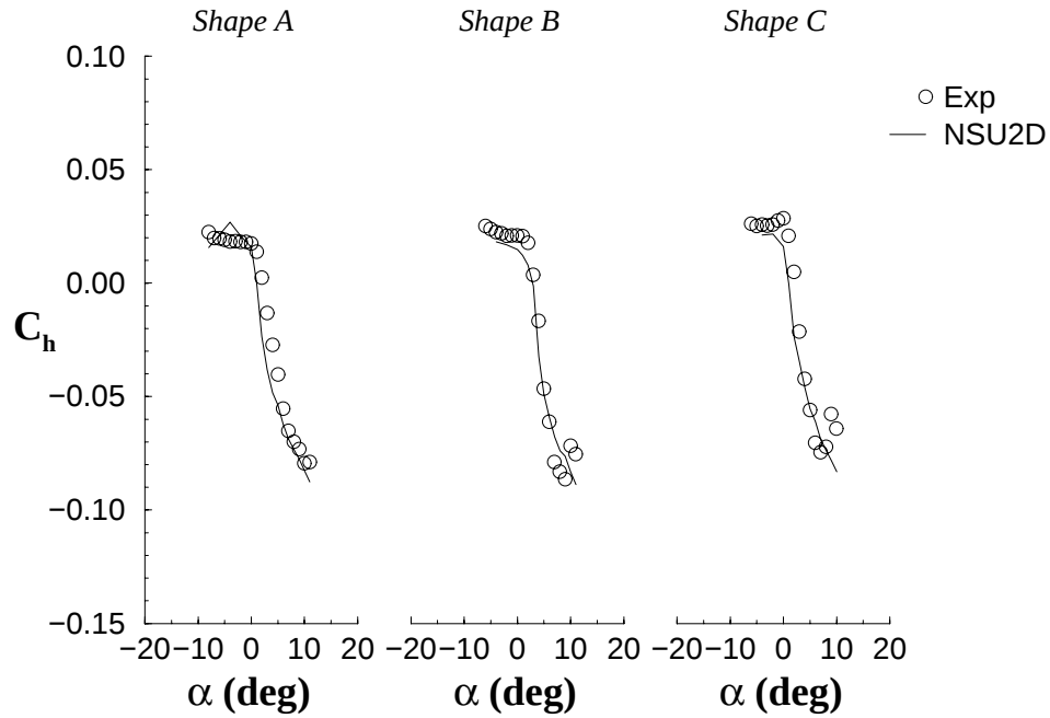
FIGURE 108. EFFECT OF ICE SHAPE GEOMETRY ON HINGE MOMENT FOR k/c = 0.0139 ICE SHAPES LOCATED AT x/c = 0.1
