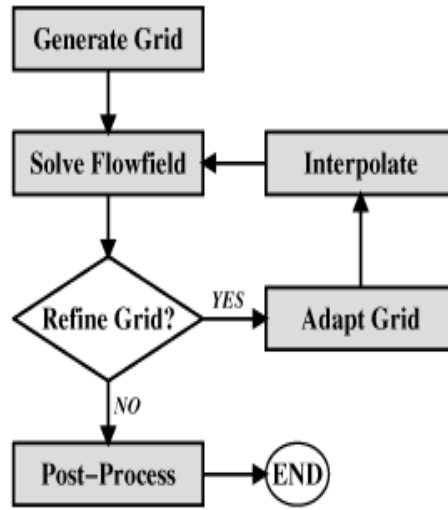
FIGURE 9. FLOWCHART OF THE OVERALL COMPUTATIONAL STRATEGY
