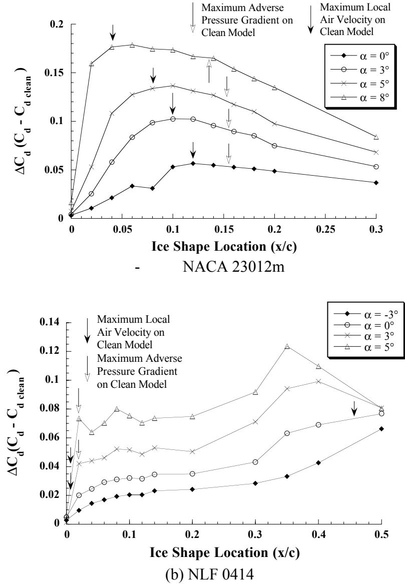
FIGURE 78. DRAG INCREASE DUE TO ICE SHAPE (0.25" forward-facing quarter round, Re = 1.8 \times 10^6 , boundary layer tripped)
