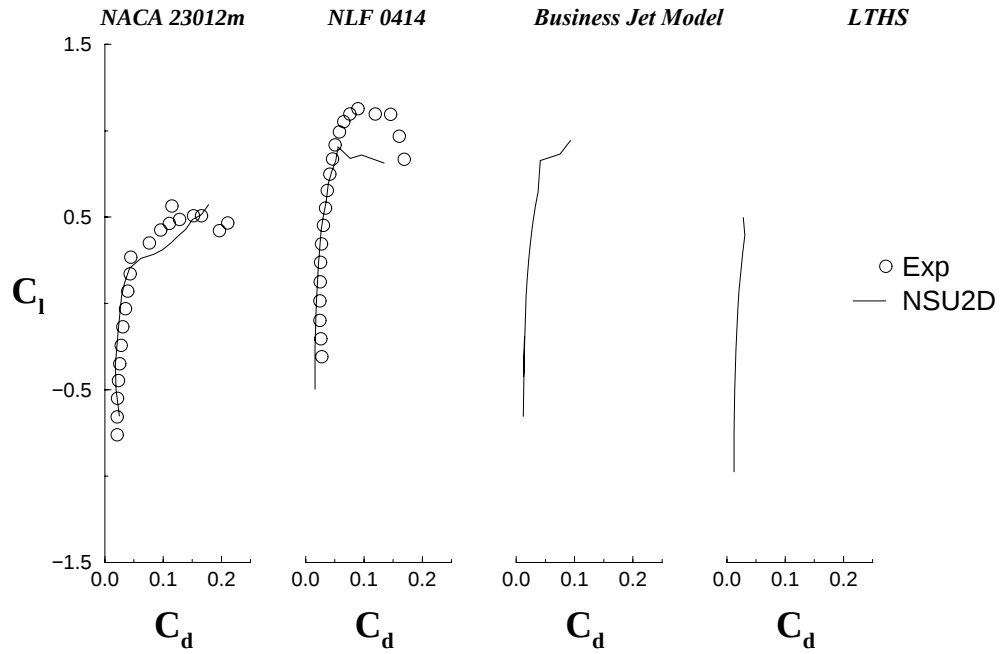
FIGURE 151. EFFECT OF AIRFOIL GEOMETRY ON DRAG FOR k/c = 0.0083 ICE SHAPE LOCATED AT x/c = 0.1
