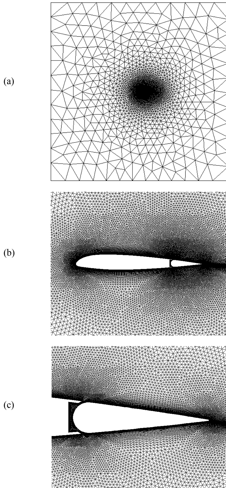
FIGURE 31. MESH FOR NACA 23012m, (a) FAR FIELD, (b) CLOSEUP, AND (c) FLAP
