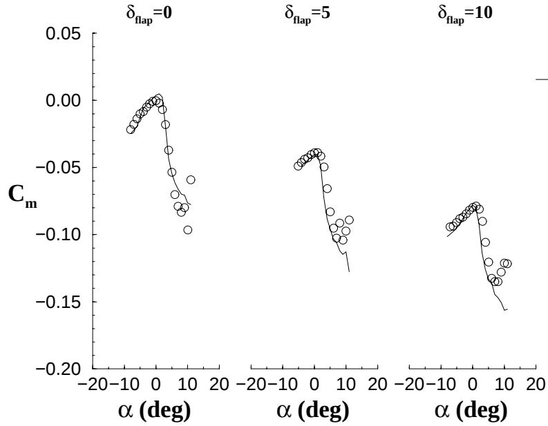
FIGURE 115. EFFECT OF FLAP DEFLECTION ON PITCHING MOMENT FOR ICED CASE WITH k/c = 0.0083 LOCATED AT x/c = 0.1
