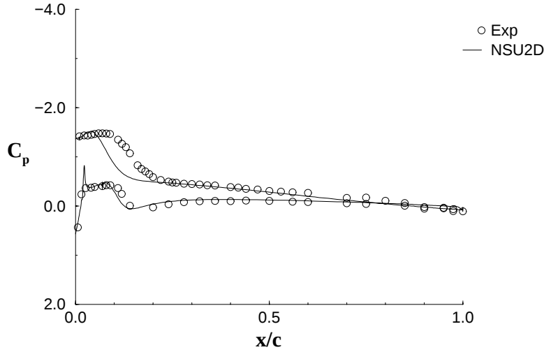
FIGURE 52. SURFACE PRESSURE DISTRIBUTION FOR A NACA 0012m AIRFOIL WITH LEADING-EDGE GLAZE ICE AT \alpha = 4.12^\circ
