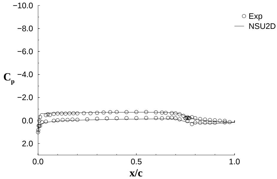
FIGURE 122. SURFACE PRESSURE DISTRIBUTION FOR A CLEAN NLF 0414 AIRFOIL FOR AN EQUIVALENT C_\ell = 0.5 AT \alpha = 0^\circ
