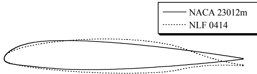
FIGURE 71. COMPARISON OF NACA 23012m AND NLF 0414 GEOMETRY
