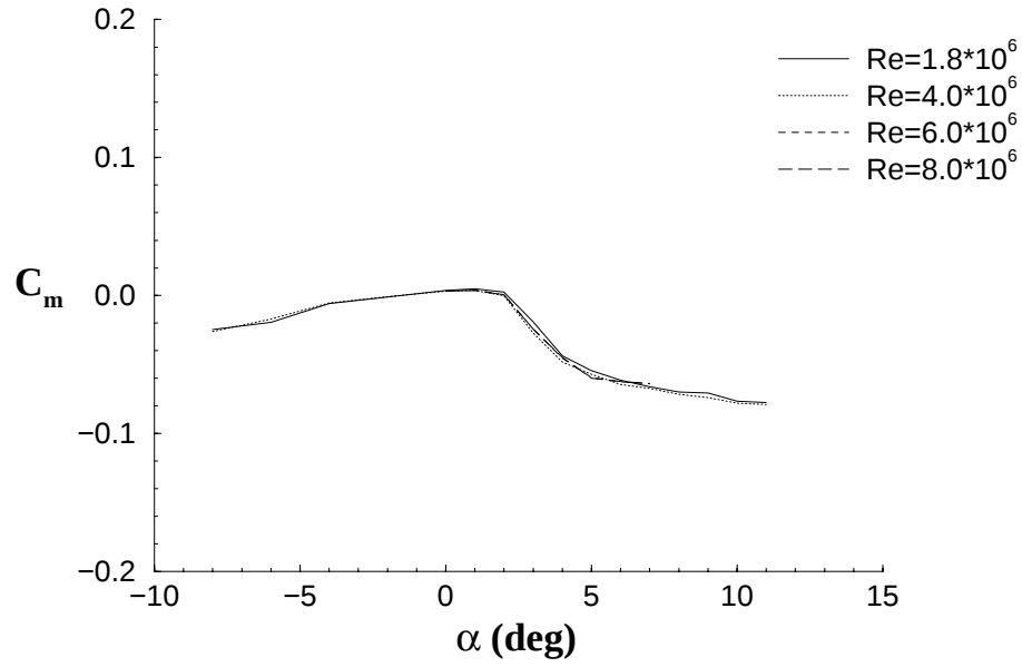
FIGURE 119. EFFECT OF REYNOLDS NUMBER ON PITCHING MOMENT FOR k/c = 0.0083 ICE SHAPE LOCATED AT x/c = 0.1
