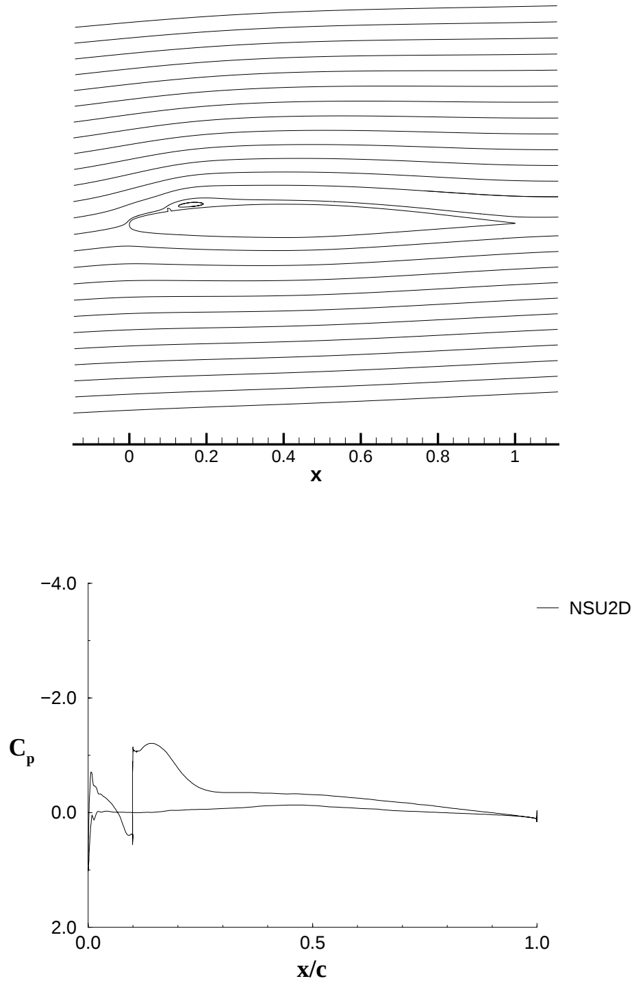
FIGURE 156. STREAMLINES AND SURFACE PRESSURE DISTRIBUTIONS FOR A BUSINESS JET MODEL AIRFOIL WITH k/c = 0.0083 QUARTER-ROUND ICE SHAPE LOCATED AT x/c = 0.1 AND \alpha = 2^\circ
