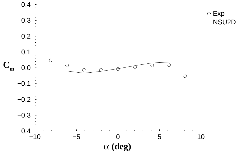
FIGURE 51. MOMENT COEFFICIENTS FOR A NACA 0012m AIRFOIL WITH LEADING-EDGE GLAZE ICE
