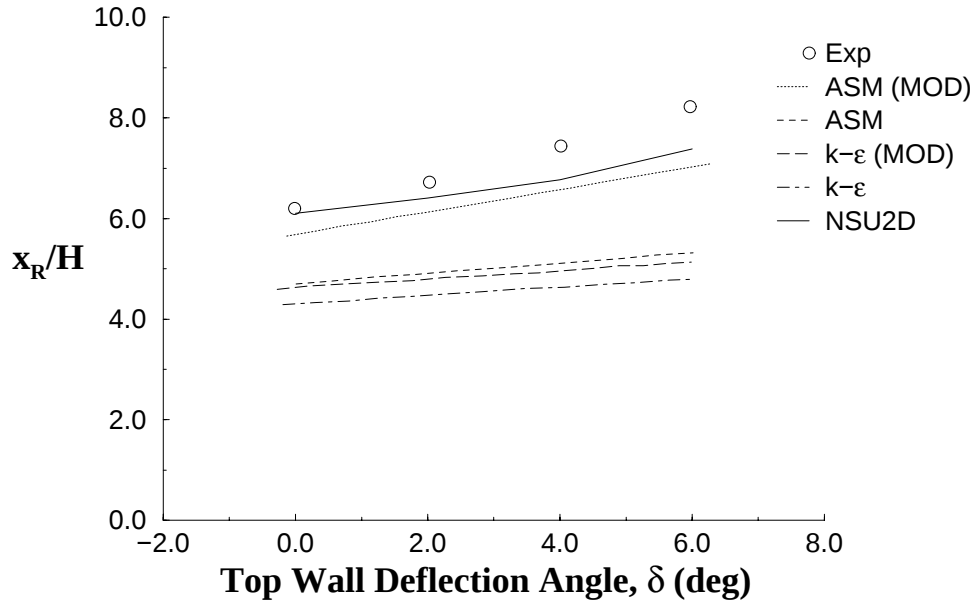
FIGURE 21. REATTACHMENT LENGTH PAST A BACKWARD-FACING STEP
