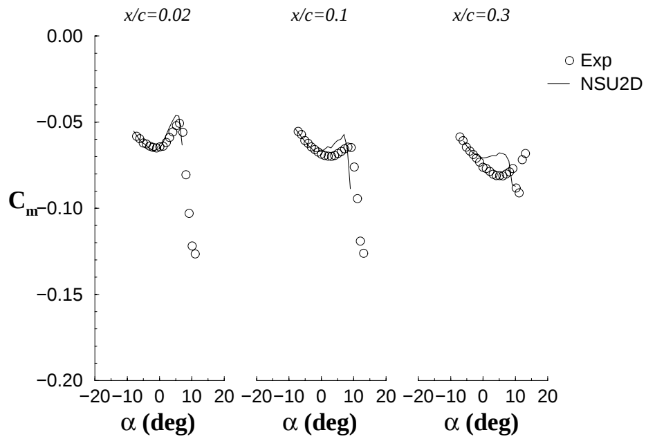
FIGURE 127. EFFECT OF ICE SHAPE LOCATION ON PITCHING MOMENT FOR k/c = 0.0083 ICE SHAPES FOR THE NLF AIRFOIL
