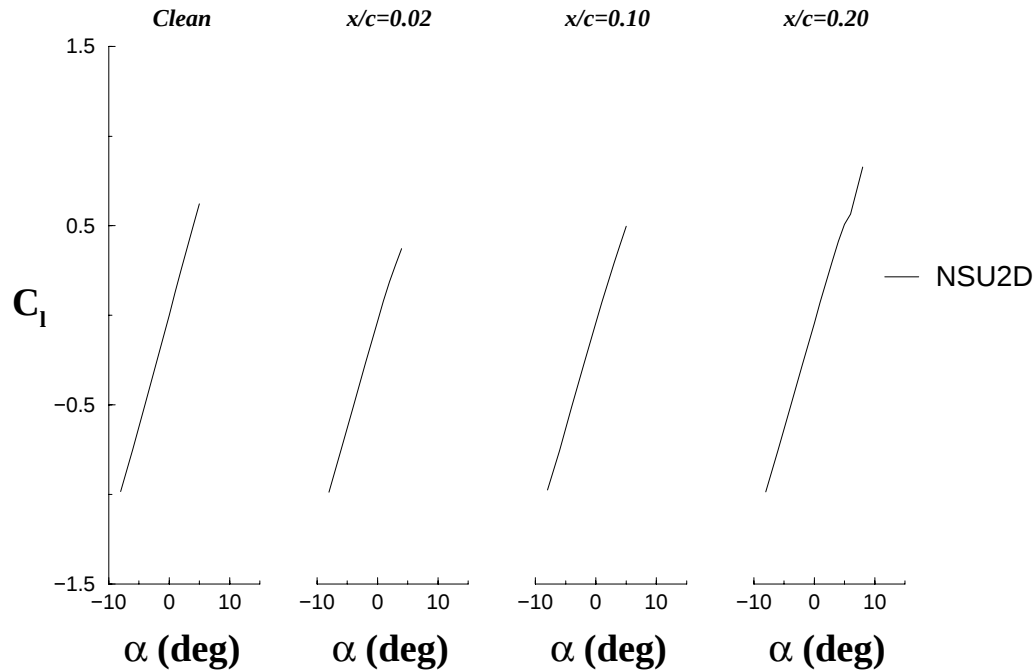
FIGURE 145. EFFECT OF ICE SHAPE LOCATION ON LIFT FOR k/c = 0.0083 ICE SHAPES FOR THE LARGE TRANSPORT HORIZONTAL STABILIZER
