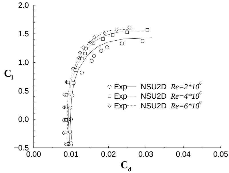
FIGURE 24. EFFECT OF VARIATION IN REYNOLDS NUMBER ON DRAG FOR A NACA 0012 AIRFOIL AT MACH NUMBER 0.15
