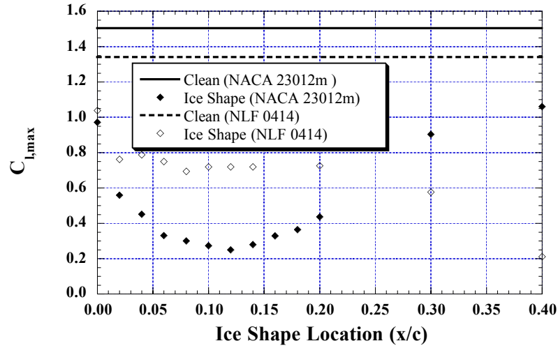
FIGURE 74. SUMMARY OF C_{\ell,max} WITH 0.25" FORWARD-FACING QUARTER ROUND SIMULATED ICE SHAPE AT VARIOUS CHORDWISE LOCATIONS ( Re = 1.8 \times 10^6 )
