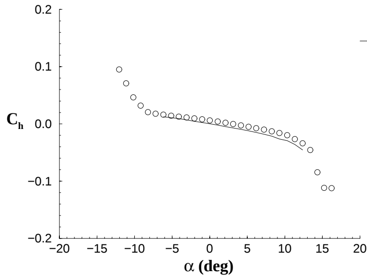
FIGURE 35. HINGE MOMENT COEFFICIENTS FOR A NACA 23012m AIRFOIL
