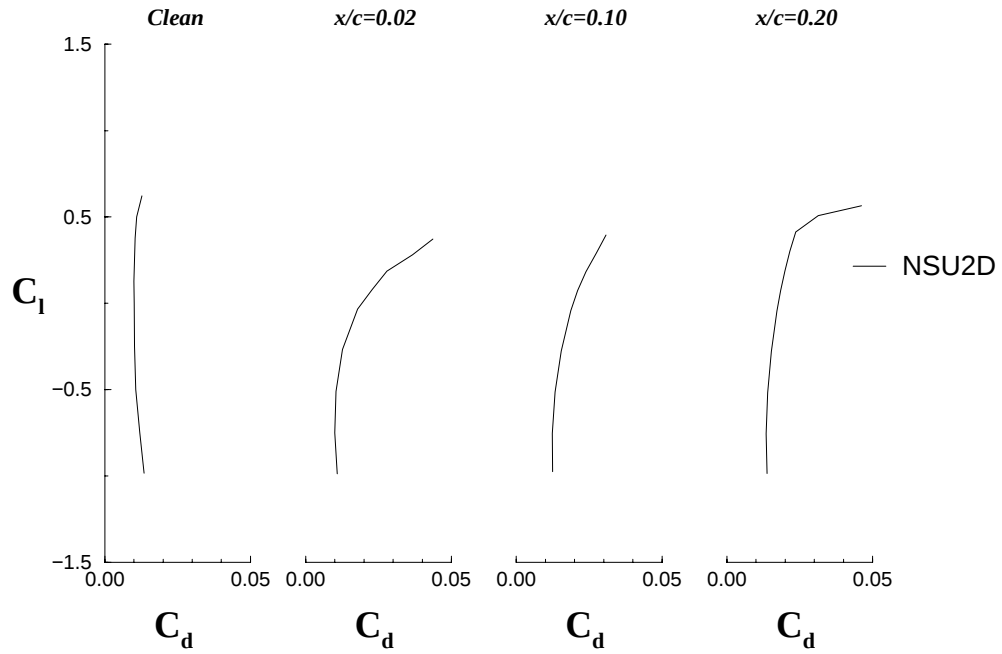
FIGURE 146. EFFECT OF ICE SHAPE LOCATION ON DRAG FOR k/c = 0.0083 ICE SHAPES FOR THE LARGE TRANSPORT HORIZONTAL STABILIZER
