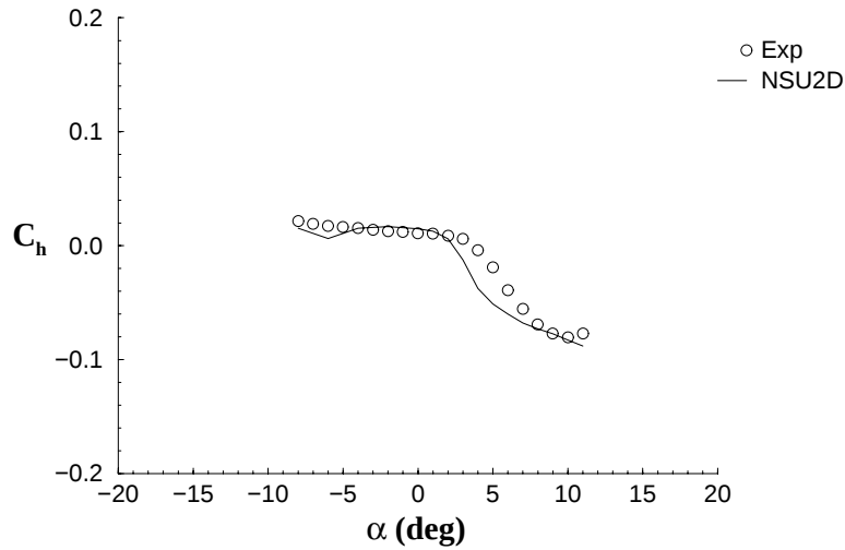
FIGURE 84. HINGE MOMENT COEFFICIENTS FOR A NACA 23012m WITH k/c = 0.0083 QUARTER-ROUND ICE SHAPE LOCATED AT x/c = 0.1
