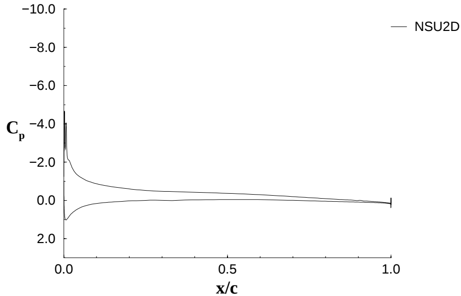
FIGURE 124. SURFACE PRESSURE DISTRIBUTION FOR A CLEAN LARGE TRANSPORT HORIZONTAL STABILIZER AIRFOIL FOR AN EQUIVALENT C_\ell = 0.5 AT \alpha = 4^\circ
