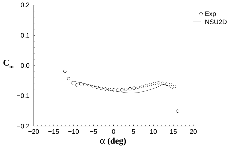
FIGURE 45. PITCHING MOMENT COEFFICIENTS FOR A NLF 0414 AIRFOIL MODELED WITH TUNNEL WALLS
