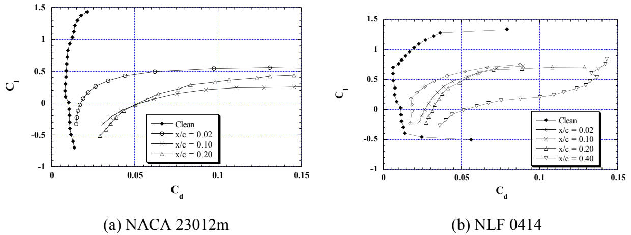
FIGURE 75. EFFECT OF SIMULATED ICE SHAPE LOCATION ON DRAG (0.25" forward-facing quarter round, Re = 1.8 \times 10^6 , boundary layer tripped)
