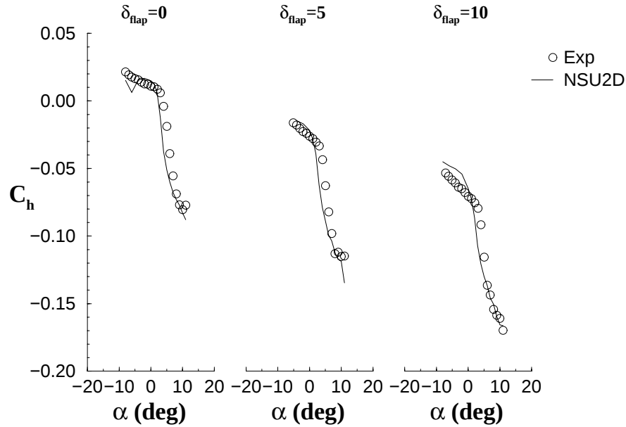
FIGURE 116. EFFECT OF FLAP DEFLECTION ON HINGE MOMENT FOR ICED CASE WITH k/c = 0.0083 LOCATED AT x/c = 0.1
