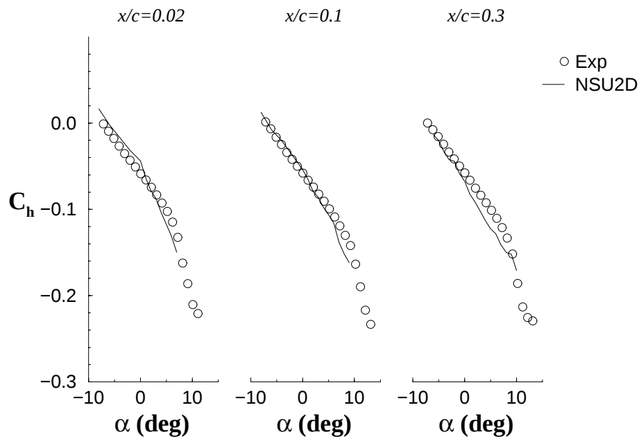
FIGURE 128. EFFECT OF ICE SHAPE LOCATION ON HINGE MOMENT FOR k/c = 0.0083 ICE SHAPES FOR THE NLF AIRFOIL
