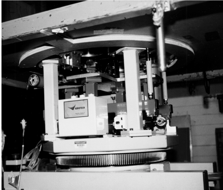
FIGURE 5. THREE-COMPONENT FORCE BALANCE
