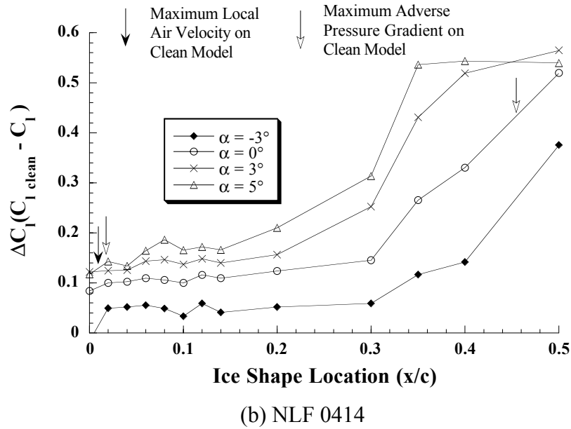
FIGURE 79. LIFT LOSS DUE TO ICE SHAPE (0.25" forward-facing quarter round, Re = 1.8 \times 10^6 , boundary layer tripped)
