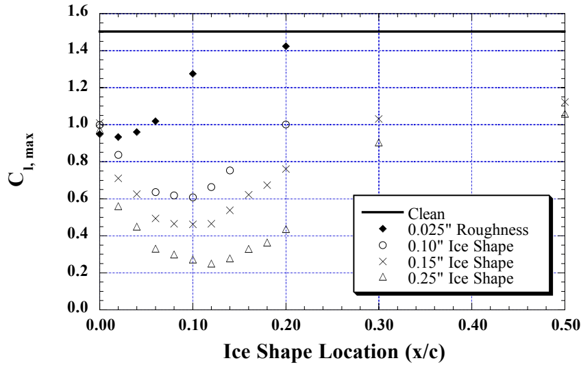
FIGURE 65. SUMMARY OF C_{l,max} WITH VARIOUS SIMULATED ICE SHAPE SIZE AND LOCATIONS (NACA 23012, forward-facing quarter round, boundary layer tripped for case with simulated ice at x/c \geq 0.04 , Re = 1.8 million)
