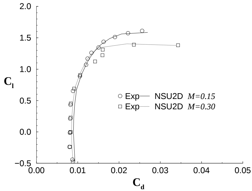
FIGURE 27. EFFECT OF VARIATION IN MACH NUMBER ON DRAG FOR A NACA 0012 AIRFOIL AT REYNOLDS NUMBER 6 MILLION
