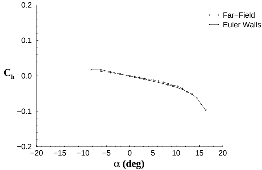
FIGURE 42. HINGE MOMENT COEFFICIENTS FOR A NACA 23012m AIRFOIL MODELED WITH TUNNEL WALLS (AND CORRECTED USING THE THEORY OF RAE AND POPE) AND WITHOUT TUNNEL WALLS
