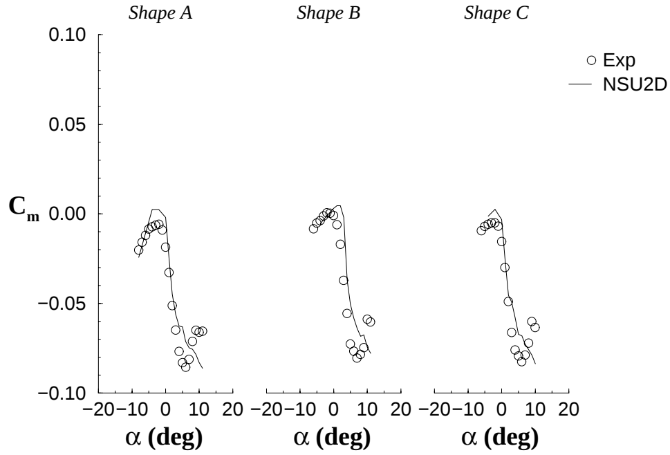
FIGURE 107. EFFECT OF ICE SHAPE GEOMETRY ON PITCHING MOMENT FOR k/c = 0.0139 ICE SHAPES LOCATED AT x/c = 0.1
