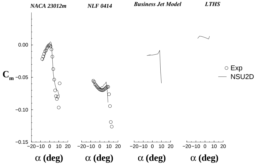
FIGURE 152. EFFECT OF AIRFOIL GEOMETRY ON PITCHING MOMENT FOR k/c = 0.0083 ICE SHAPE LOCATED AT x/c = 0.1
