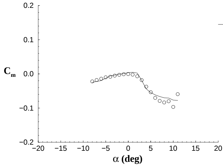
FIGURE 83. PITCHING MOMENT COEFFICIENTS FOR A NACA 23012m WITH k/c = 0.0083 QUARTER-ROUND ICE SHAPE LOCATED AT x/c = 0.1
