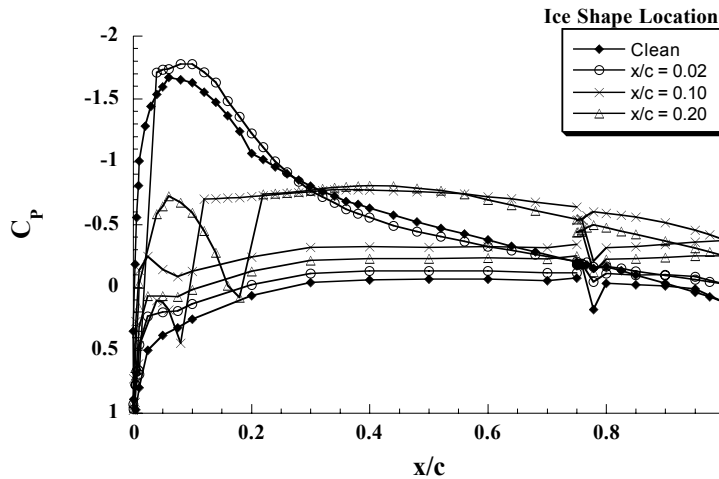
(b) \alpha = 5^\circ
