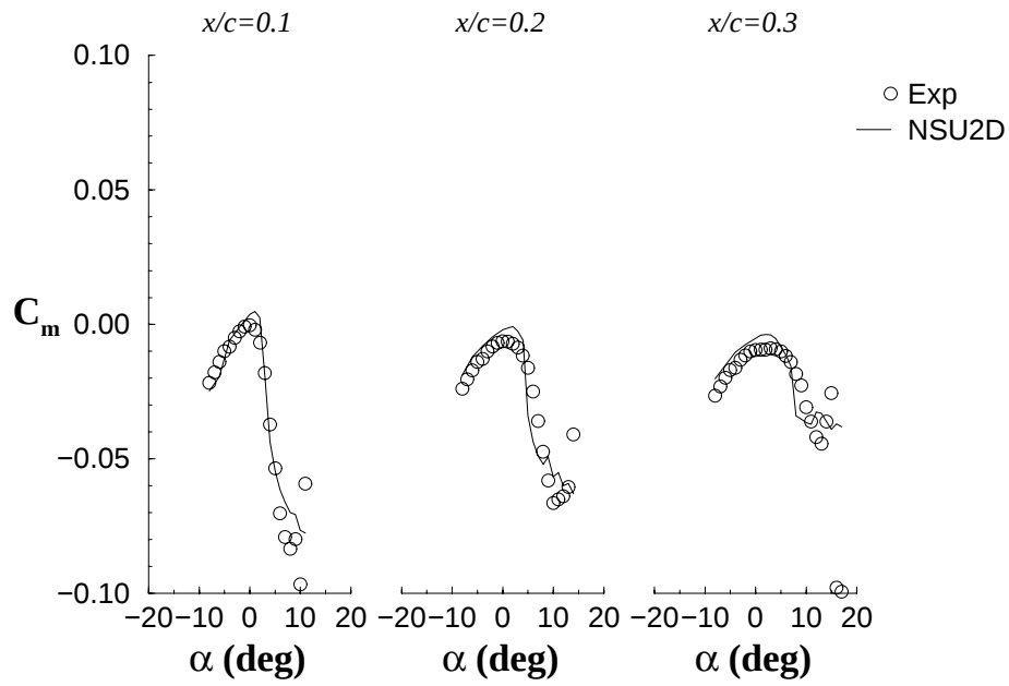
FIGURE 98. EFFECT OF SHAPE LOCATION ON PITCHING MOMENT FOR k/c = 0.0083 ICE SHAPE
