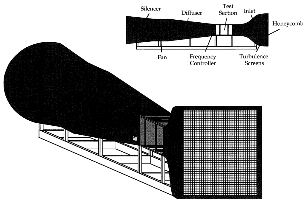
FIGURE 3. UNIVERSITY OF ILLINOIS 3' \times 4' SUBSONIC WIND TUNNEL
