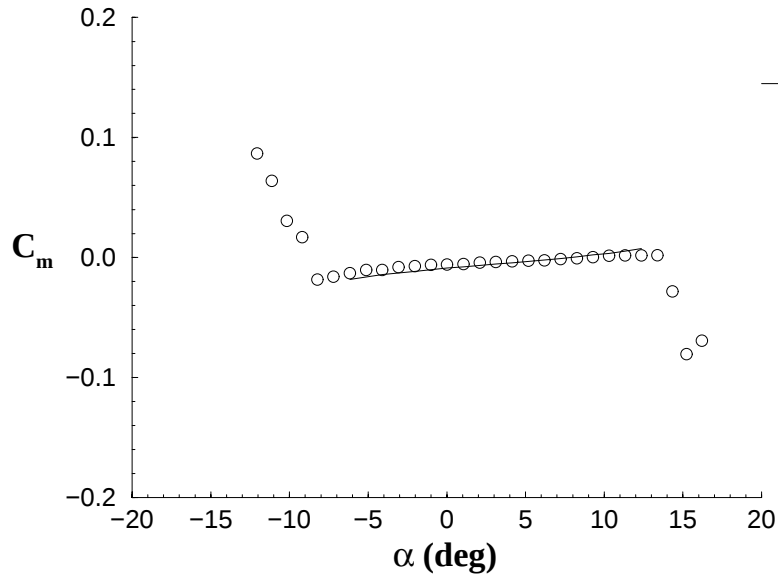
FIGURE 34. PITCHING MOMENT COEFFICIENTS FOR A NACA 23012m AIRFOIL
