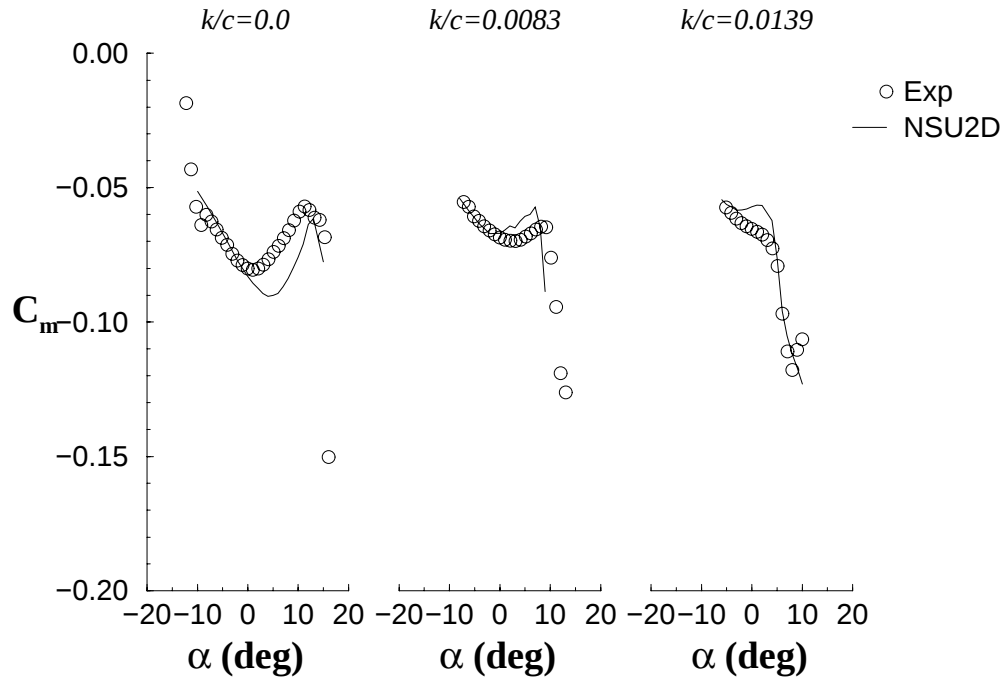
FIGURE 135. EFFECT OF ICE SHAPE HEIGHT ON PITCHING MOMENT FOR A NLF AIRFOIL WITH A QUARTER-ROUND ICE SHAPE LOCATED AT x/c = 0.1
