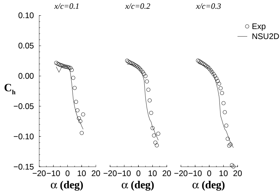
FIGURE 99. EFFECT OF SHAPE LOCATION ON HINGE MOMENT FOR k/c = 0.0083 ICE SHAPE
