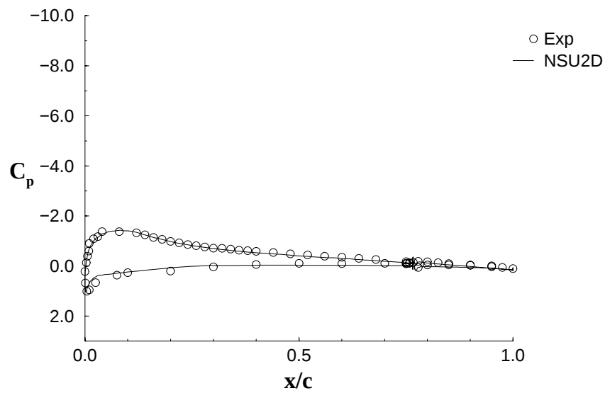
FIGURE 36. SURFACE PRESSURE DISTRIBUTION FOR A NACA 23012m AIRFOIL AT \alpha = 4.14^\circ
