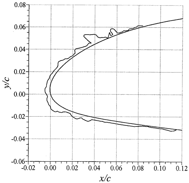
FIGURE 3. ICE ACCRETION CHARACTERISTICS FOR RUN 296, TRACING FROM RUN 293 (REPEAT RUN), AND PHOTOGRAPH FROM RUN 296
