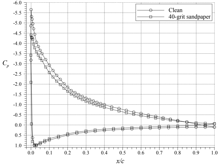
FIGURE 26. COMPARISON OF CLEAN AND 40-GRIT SANDPAPER PRESSURE DISTRIBUTIONS FOR THE NACA 23012 AIRFOIL AT \alpha = 11^\circ , Re = 7.5 \times 10^6 , AND Ma = 0.21
