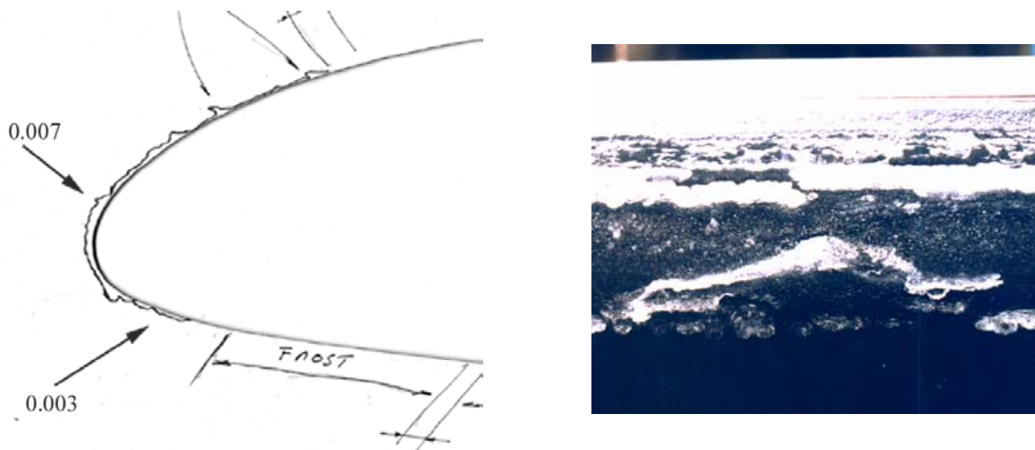
FIGURE 9. TRACING AND PHOTOGRAPH OF INTERCYCLE ICE RUN 326. CLOUD CONDITIONS SAME AS RUN 290, WITH 1-minute BOOT CYCLE. ROUGHNESS HEIGHTS (0.007, 0.003) NORMALIZED BY CHORD ( k/c ).
