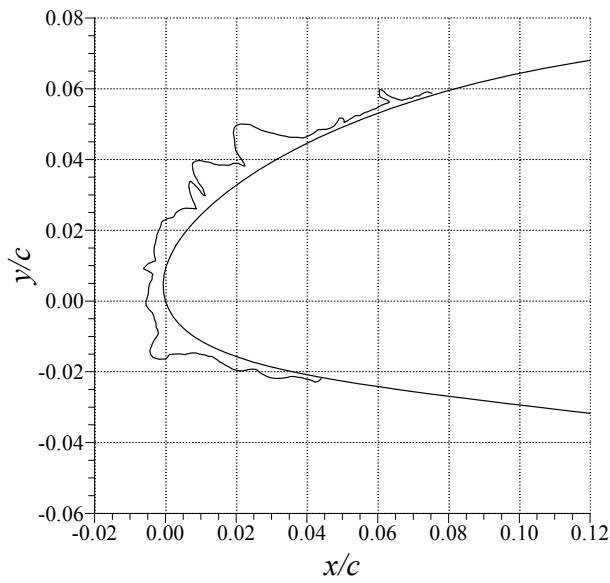
FIGURE 2. ICE ACCRETION CHARACTERISTICS FOR RUN 290, TRACING FROM RUN 288, AND PHOTOGRAPH FROM RUN 292 (REPEAT RUNS)
