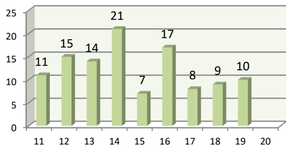
3. Collision w/Obstacles
