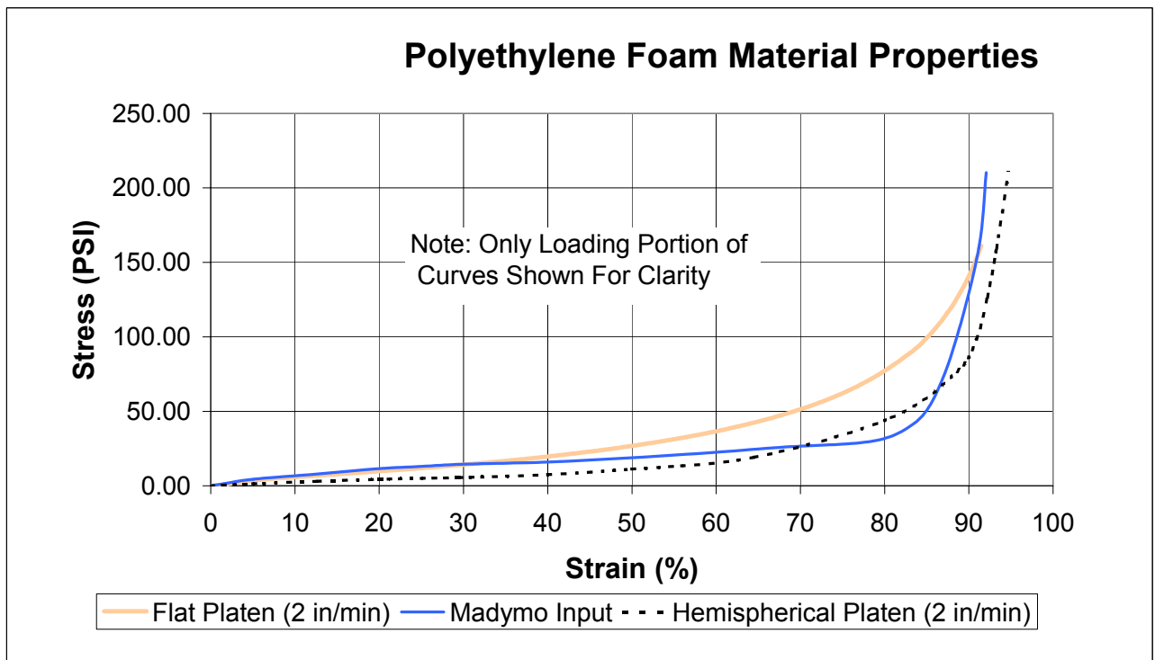
Figure 24. Foam Properties
