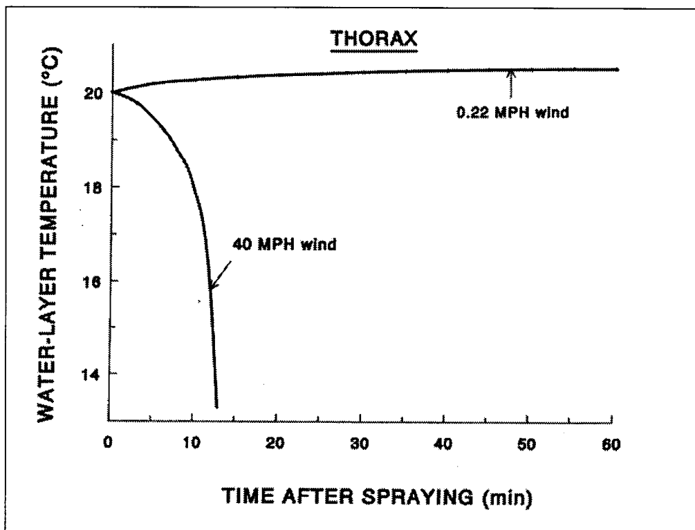
Figure 11. Temperature changes of the water layer for the conditions shown in Fig. 10.
