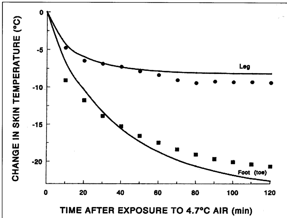
Figure 9. Comparison between experimental data (4) and model predictions for various skin temperatures during cold-air exposure.
