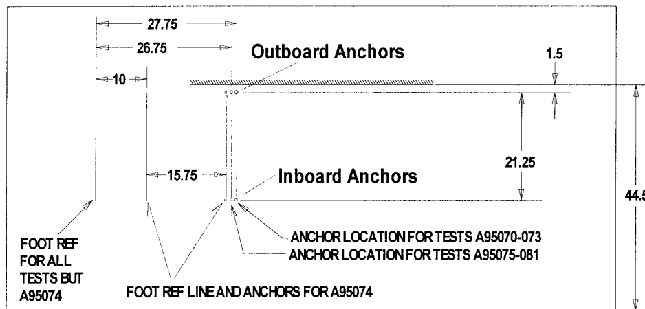
SLED TOP VIEW
