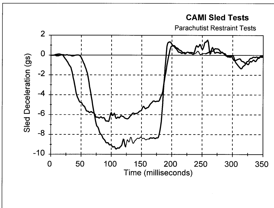
Examples of the 2 Impact Deceleration Pulses in the Project Figure 8.
