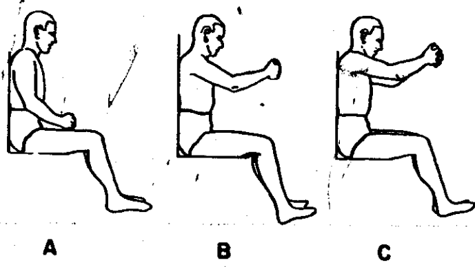
FIGURE 8. Position of body C. G. of pilot operating controls in various positions; back erect, seat 90° to back, legs 110° to thighs.
