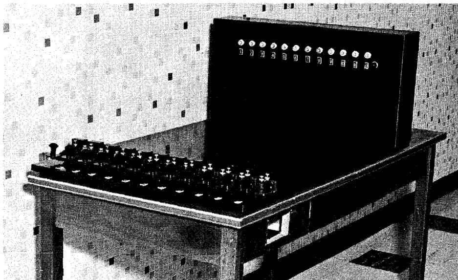
FIGURE 8. Serial-performance task.
