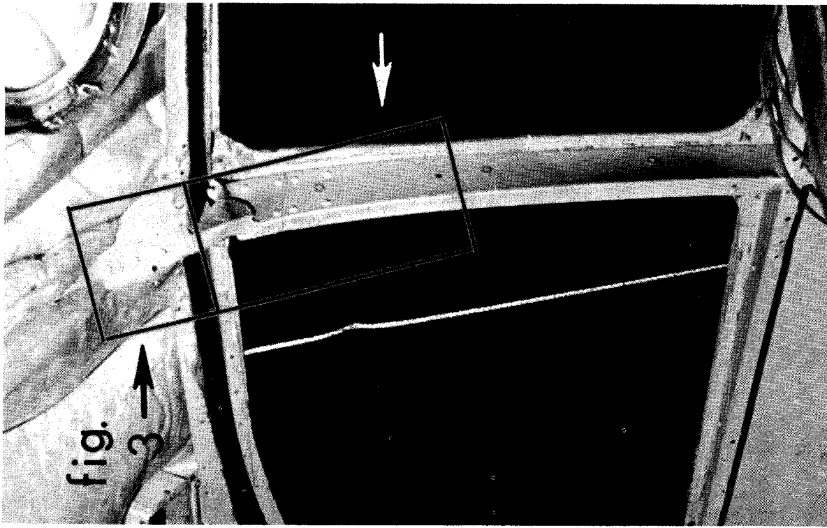
FIGURE 4. Piper : Left side view.
