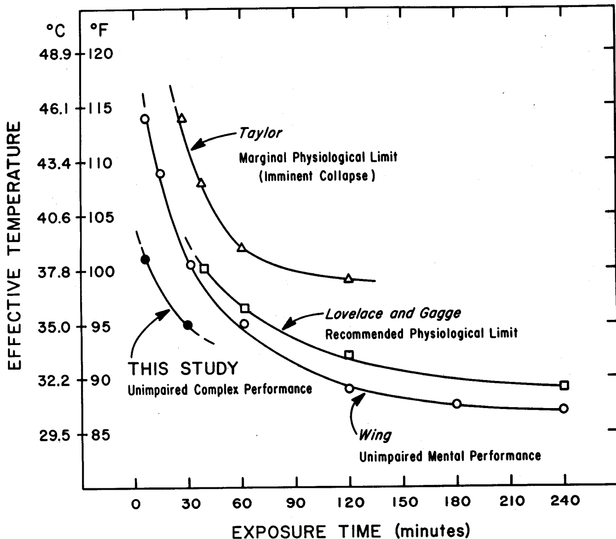
FIGURE 5—Physiological and performance limits in hot environments (modified from Wing 10 ).
