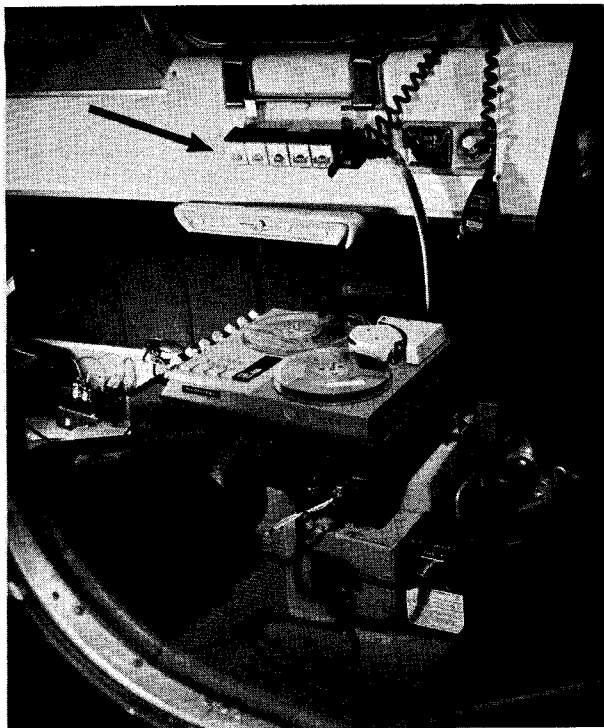
FIGURE 3. Portable, seven-channel tape recorder used to obtain in-flight pilot performance data during simulated instrument approaches. Arrow indicates meter panel for monitoring inputs to recorder.
