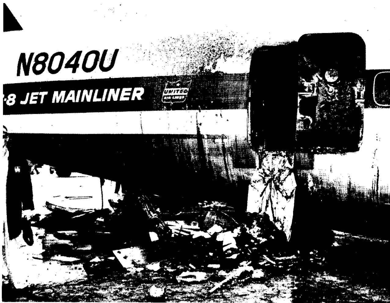
FIGURE 10. Aft galley service door of Denver DC-8 showing deflated escape slide. A total of 40 2nd-class passengers used this exit. The slide burned after approximately 20 passengers had escaped, forcing the remainder to jump.
