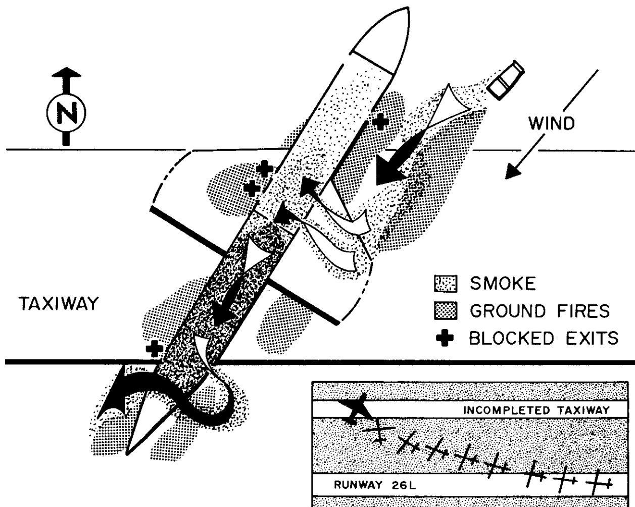
FIGURE 1. Path (inset) and final position of Denver DC-8. Smoke from ground fuel fires forward of right wing entered cabin through opened right window exits. Concentration of smoke was particularly intense in 2nd-class (aft) passenger compartment due to draft produced by open right rear galley exit.
