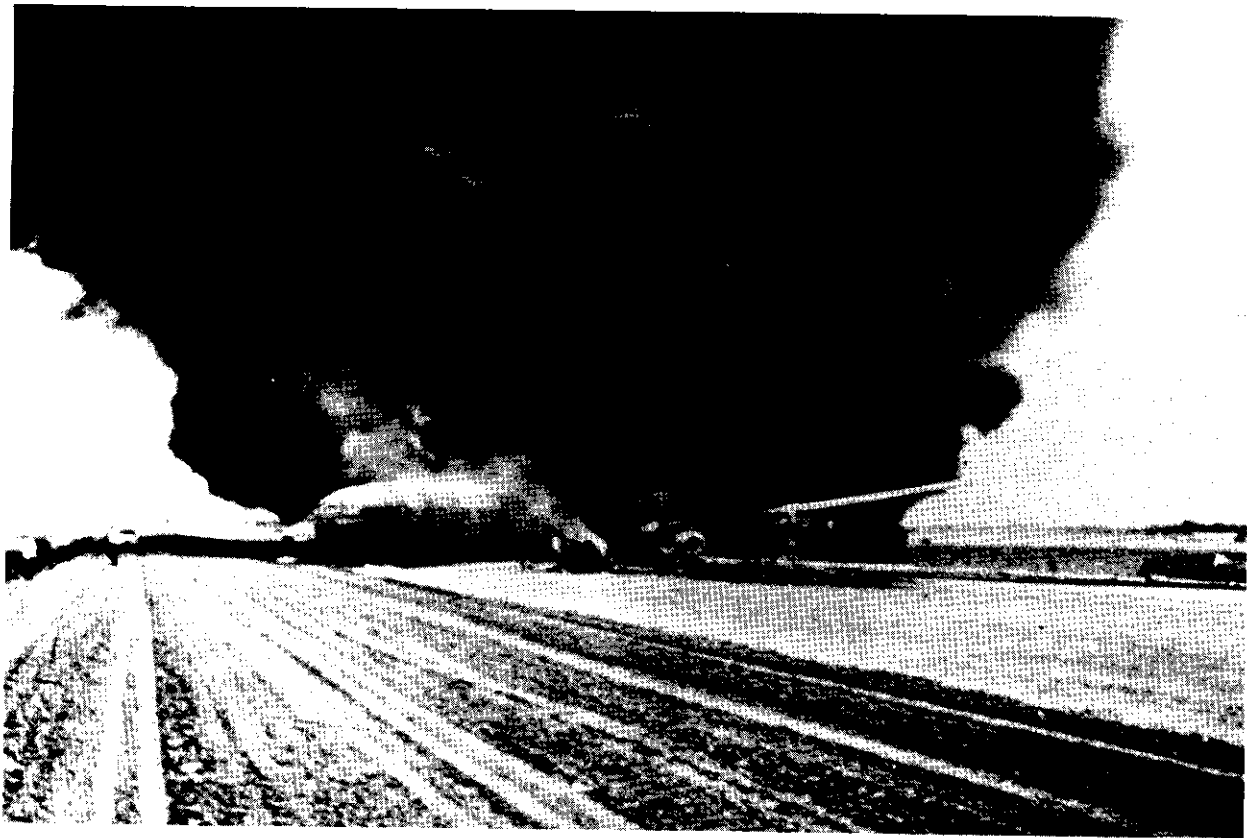
FIGURE 6. Right front view of the Denver DC-8 taken by airport employee soon after aircraft came to rest and before arrival of fire-fighting equipment. It shows the extent of outside fire and the direction of smoke dispersion.
