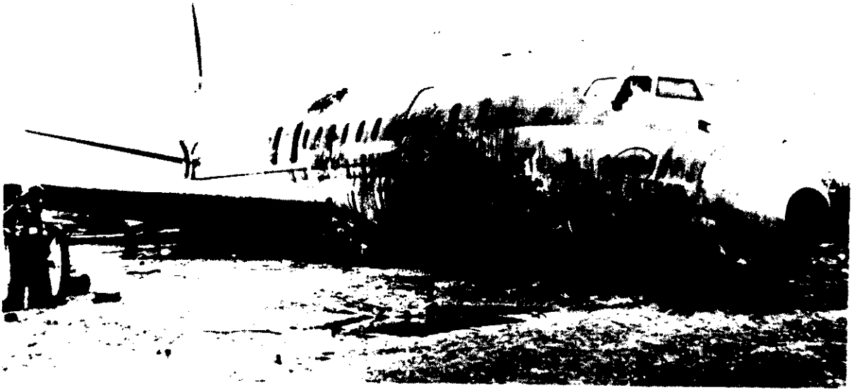
FIGURE 5. Right front view of Denver DC-8 showing the two overwing exits and right aft galley service door through which a total of 66 passengers escaped. A pool of unburned fuel is shown to the right of the cockpit. Ground fire in this area prevented use of the forward service door and a 7-knot NE wind carried smoke from this fire into the cabin through the open window exits.
