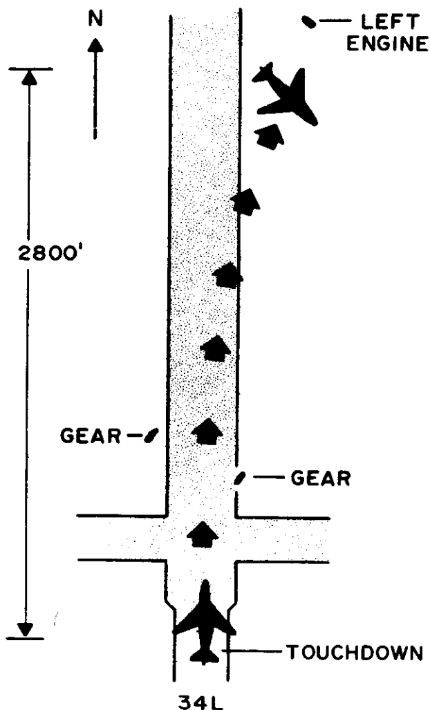
FIGURE 16. Skid path and final location of Salt Lake City 727.
