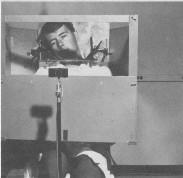
FIGURE 1. Modifications of a rotating device to control head movements and to introduce an aviation-related visual environment. The rod extending upward from the foot rest terminates in a plastic panel which contains three tiny lights (a red and a green "wing-tip" light and a flashing red "beacon") simulating an approaching aircraft. Upper left: rotation device without the "cabin" attachment (the chin rest depicted here is used for research rather than demonstration purposes). Upper right: the major section of the "cabin" has been bolted to the back of the head rest; its base is further supported by small metal extensions projecting outward from the arms of the chair. Lower left: the instrument panel is added to the "cabin" by means of four wing-nuts. Lower right: interior view of the "cabin" with a subject's head tilted to the right; the lights of the approaching aircraft were viewed through the "window" of the "cabin." The interior of the "cabin" was coated with luminous paint.
