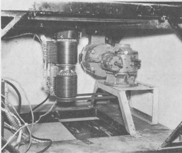
FIGURE 7. A modified Link trainer used by a flying school to provide disorientation familiarization.
