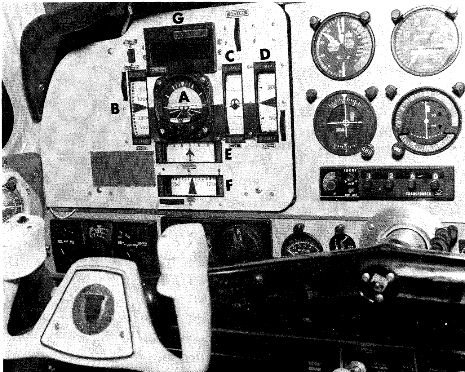
FIGURE 1. Peripheral vision flight display (PVFD), installed in Beechcraft Bonanza 35A, used to measure pilot performance during ILS approaches. A—Attitude Indicator, B—Airspeed Indicator, C—Glidepath Indicator, D—Vertical Speed Indicator, E—Localizer Indicator, F—Heading Indicator, and G—Altimeter.
