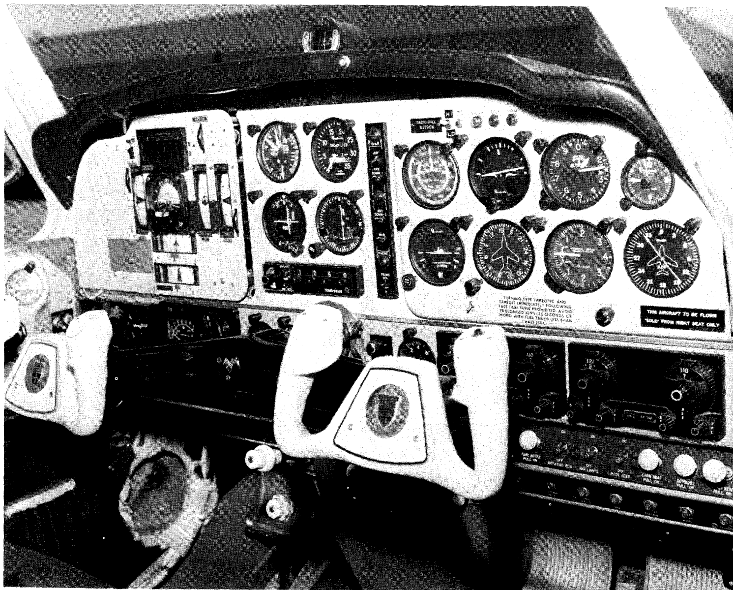
FIGURE 3. Comparison of areas occupied by peripheral vision flight display (left) and conventional panel (right).
