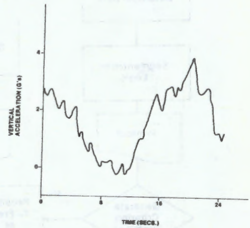
BARREL ROLL ACCELERATION/TIME PLOT
