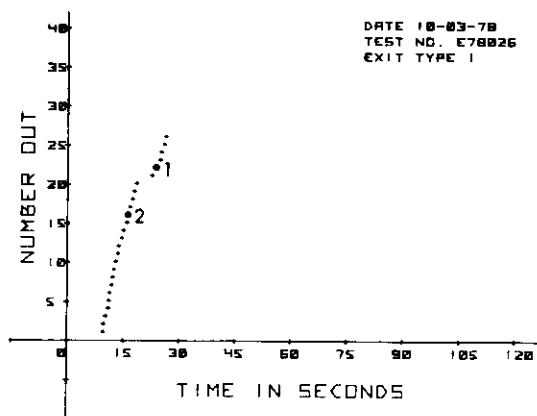
Figure 2. Data plot of evacuation test results
