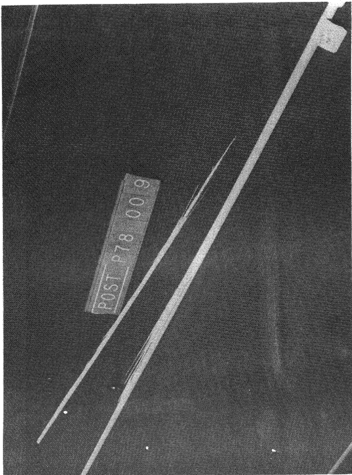
Figure 6. Typical failure mode of solid fiber-reinforced canes.
