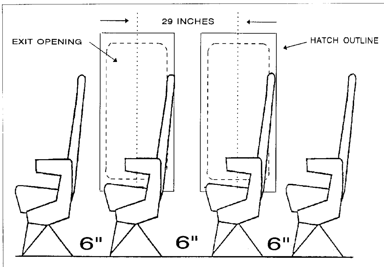
FIGURE 4. CONFIGURATION "D"
