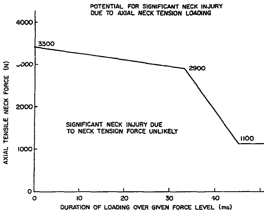
Figure 2 - Injury criterion for neck axial tension loading (Mertz, 1984)
