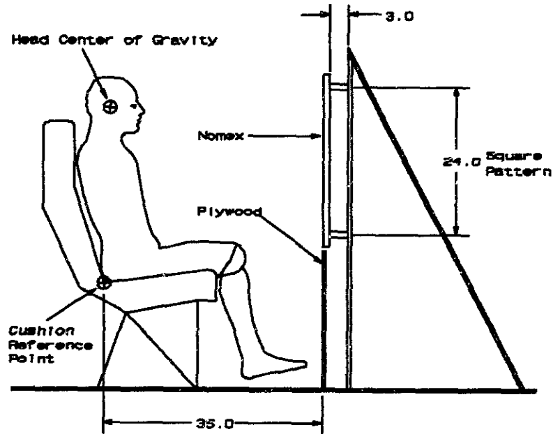
Figure 4 - Test Setup for Unpadded Nomex Honeycomb
