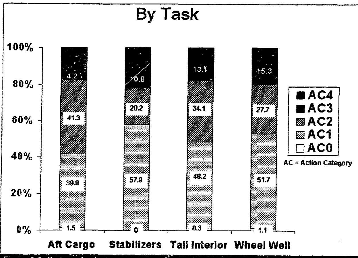
Figure 5.3. Posture Analysis
