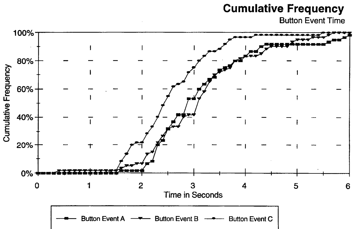
Figure 12. Cumulative frequency for button event egress times for subjects in restraints A, B, and C.
