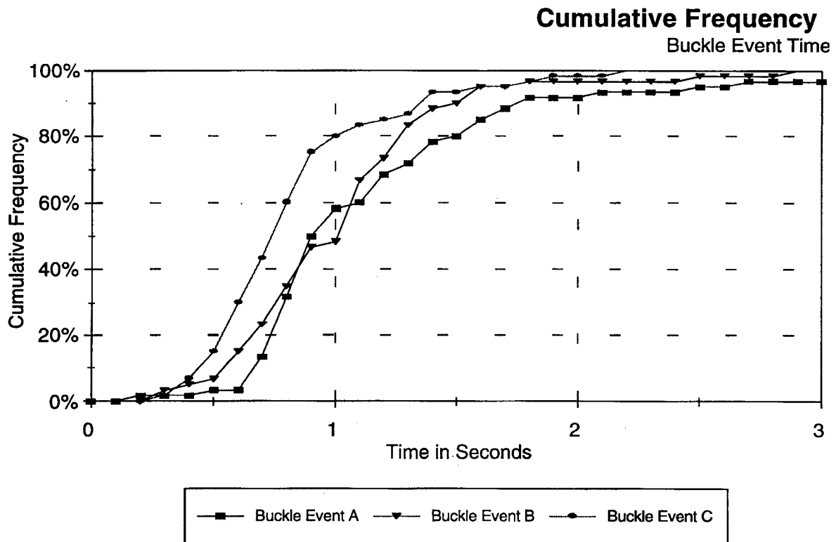
Figure 8. Cumulative frequency for release times of restraints A, B, and C.
