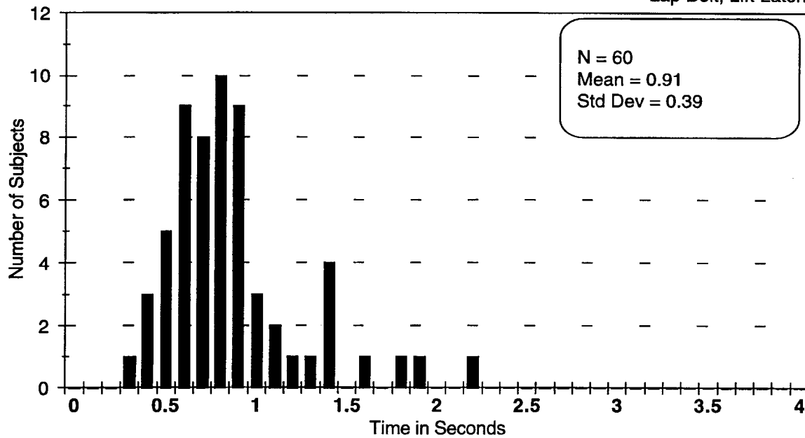
Figure 7. Buckle release time for restraint C.
