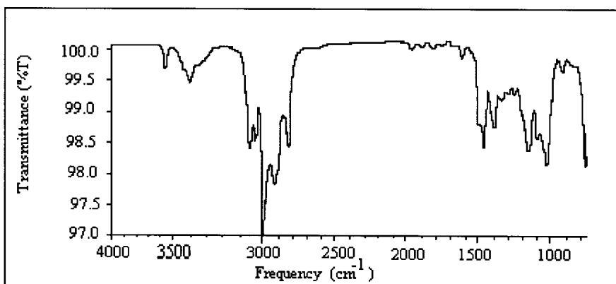
FIG. 2B —The infrared spectrum of (+)-pseudoephedrine subjected to the GC/FTIR analysis.
