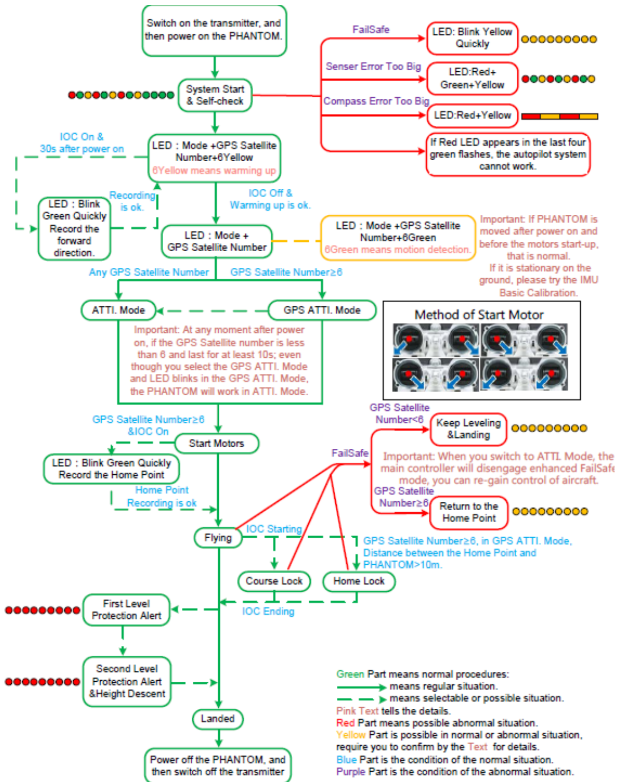
PHANTOM Flying Flowchart VI.0 (Simplified Version)
