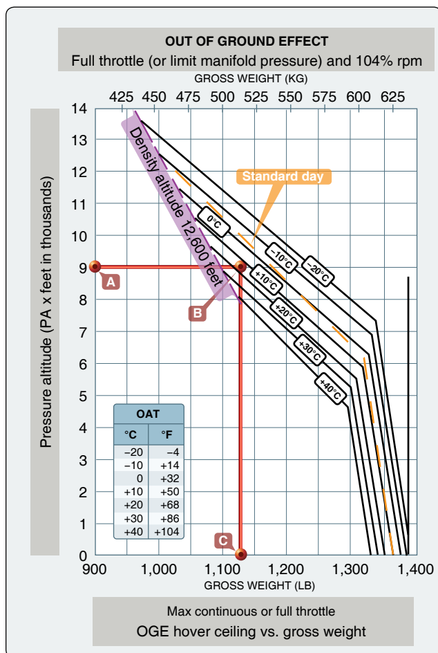
Figure 7-5. Out of ground effect hovering ceiling versus gross weight chart.
