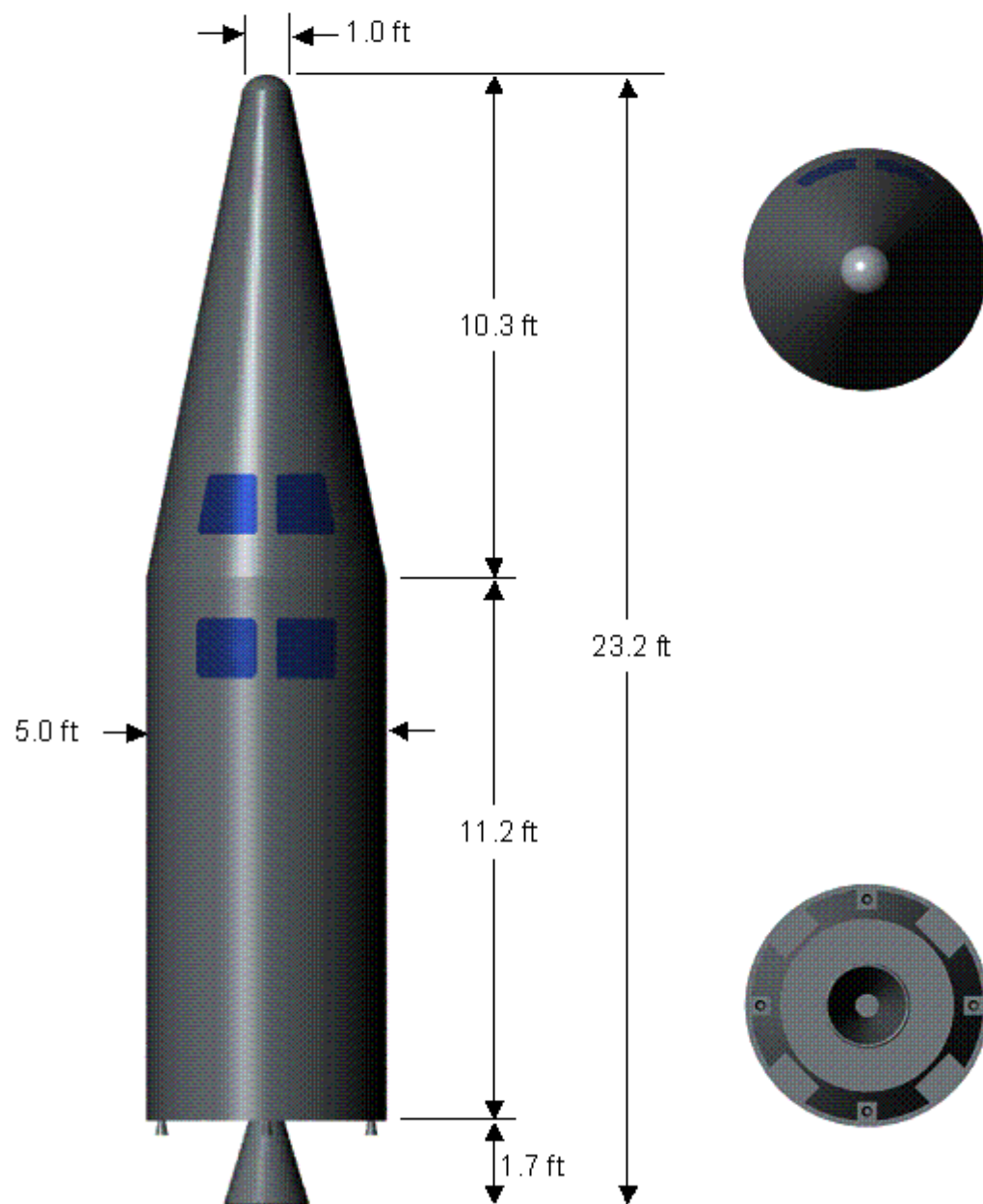
Figure 2: Vehicle Dimensions
