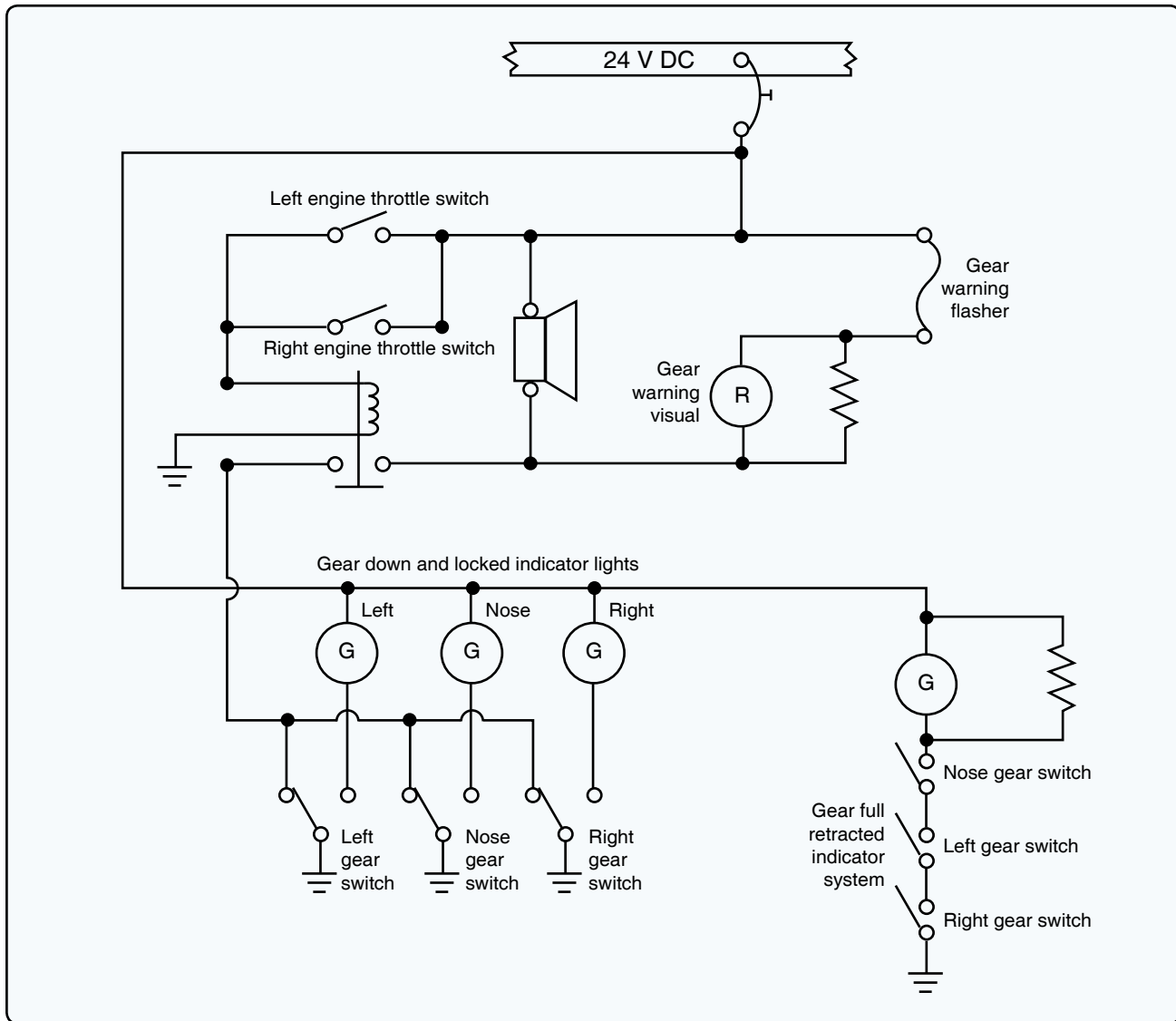
Figure 20. Landing gear circuit.
