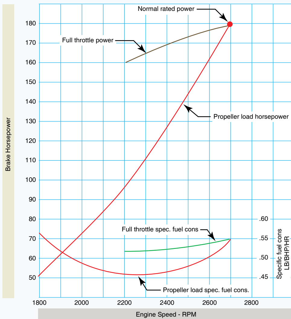
Figure 41. Performance chart.
