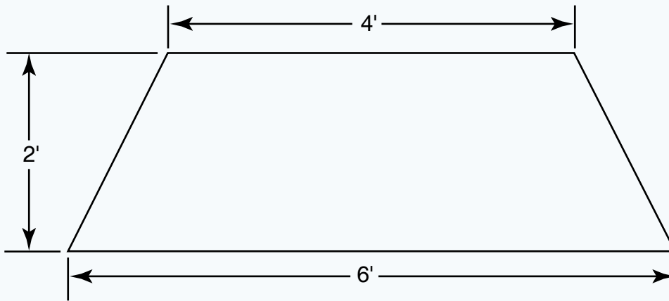
Figure 56. Trapezoid area.
