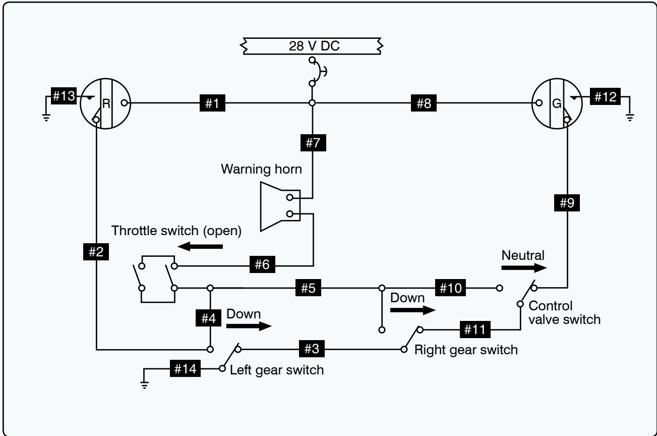
Figure 18. Landing gear circuit.
