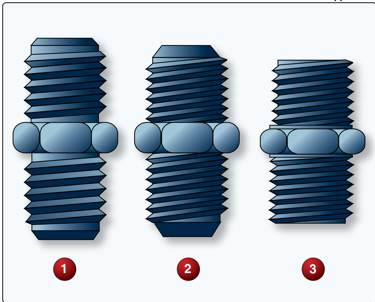
Figure 11. Fittings.
