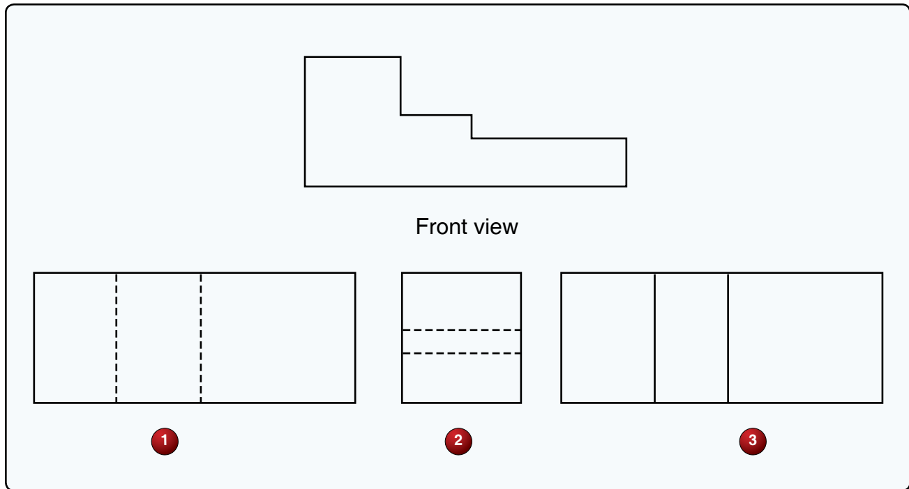
Figure 30. Object views.
