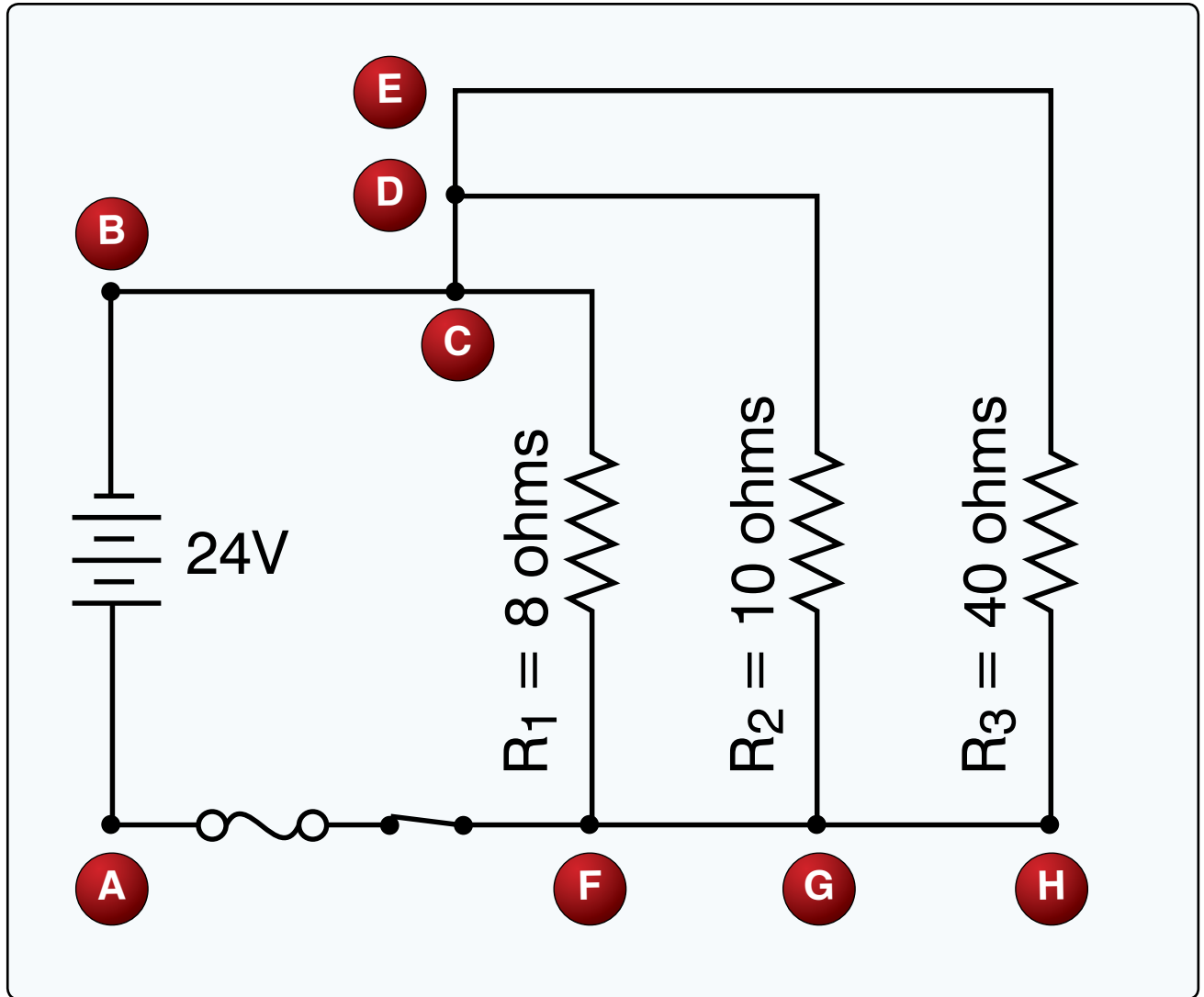
Figure 11. Circuit diagram.
