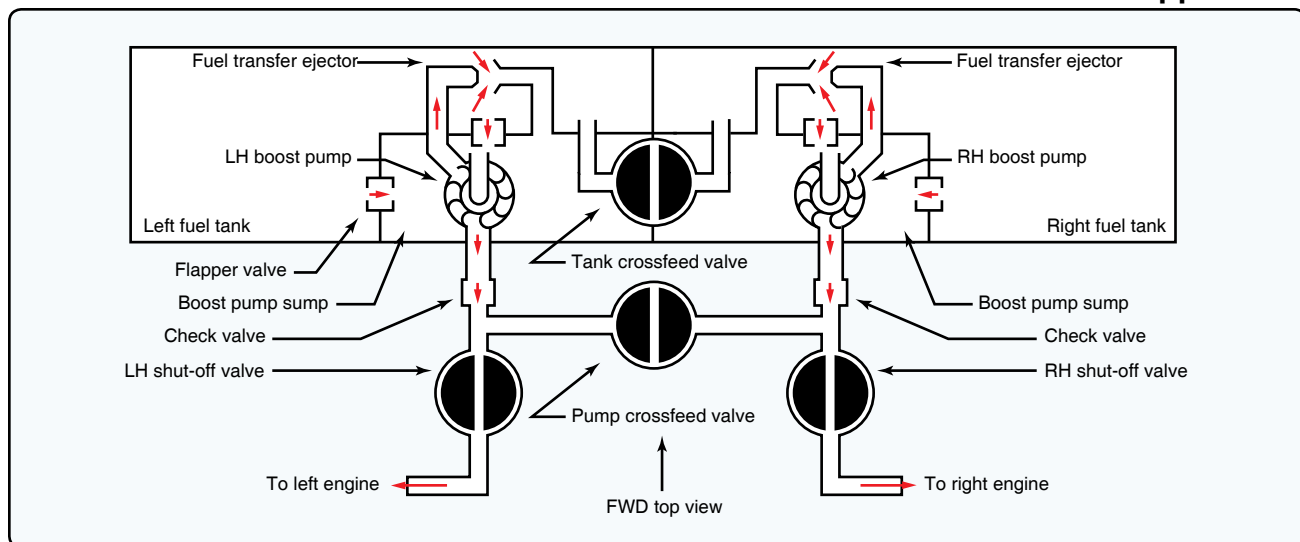
Figure 17. Fuel system.
