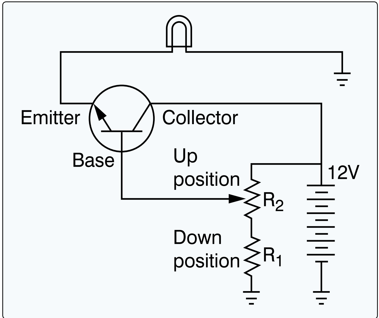
Figure 23. Transistorized circuit.
