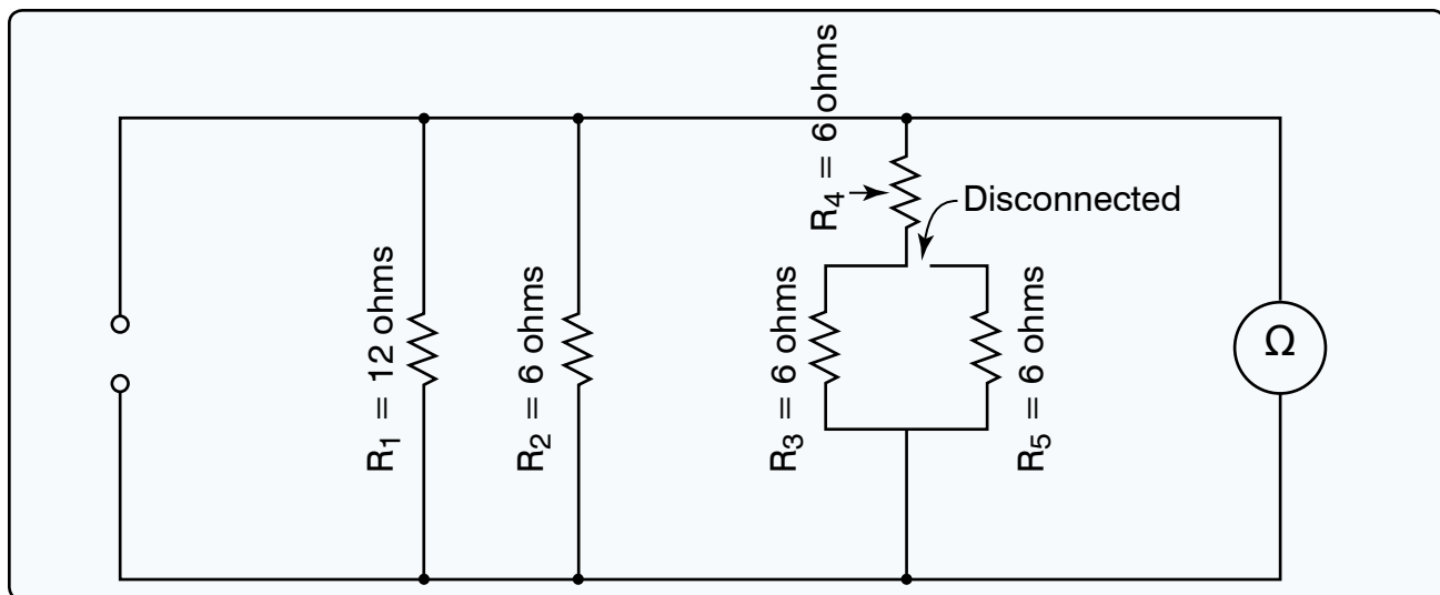
Figure 6. Circuit diagram.
