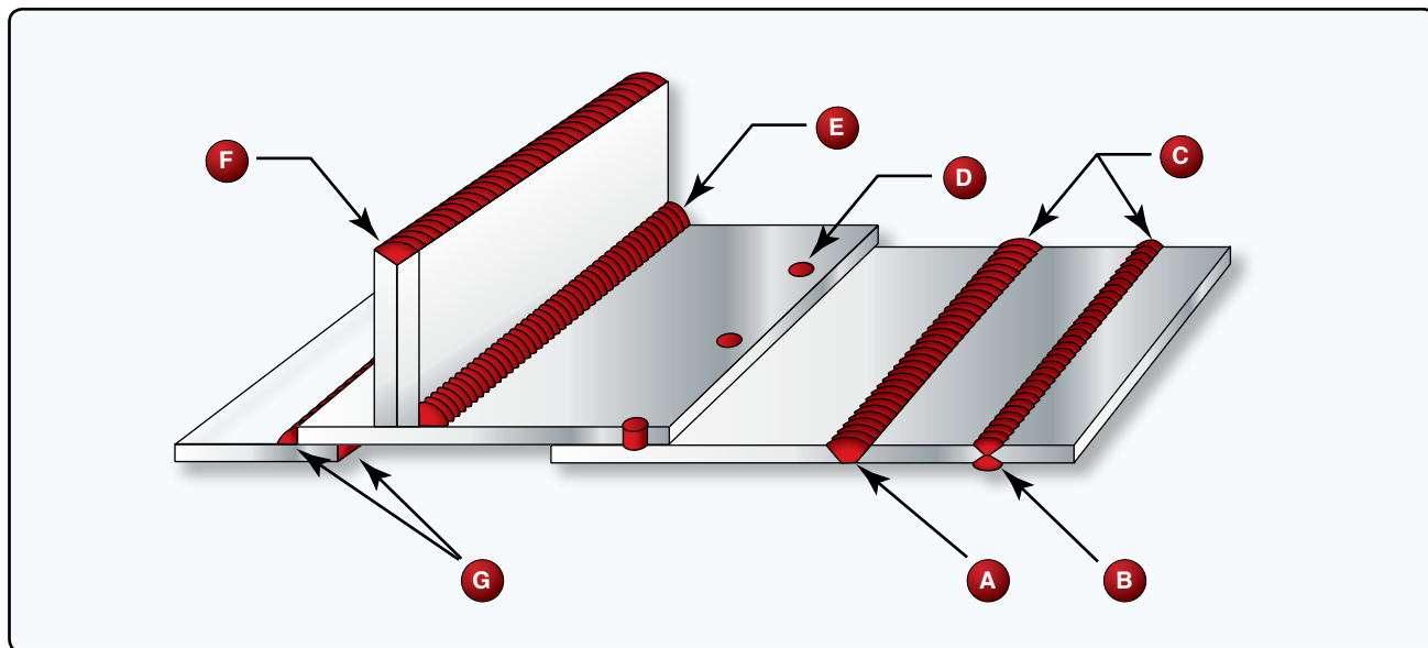
Figure 45. Welds.
