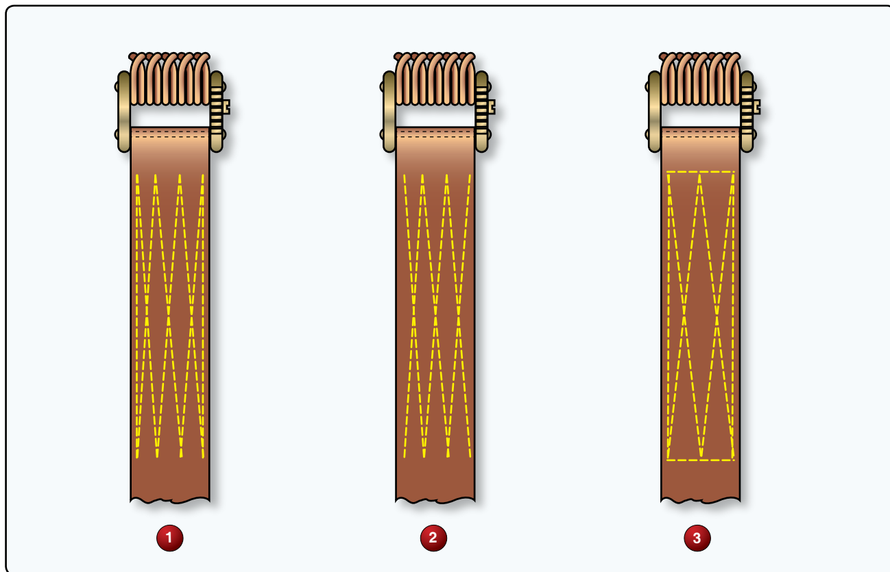
Figure 8. Lift web stitching.
