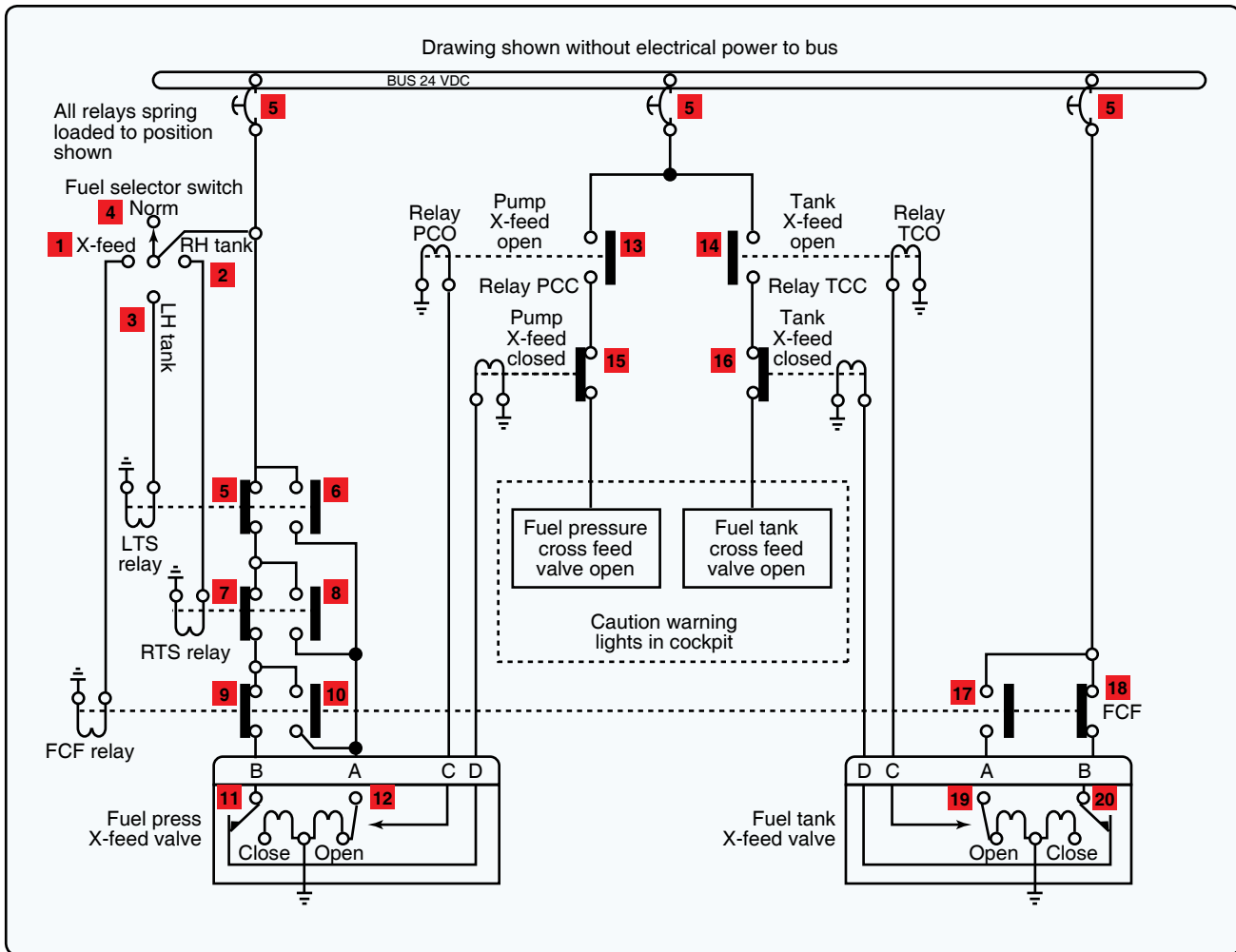
Figure 16. Fuel system circuit.
