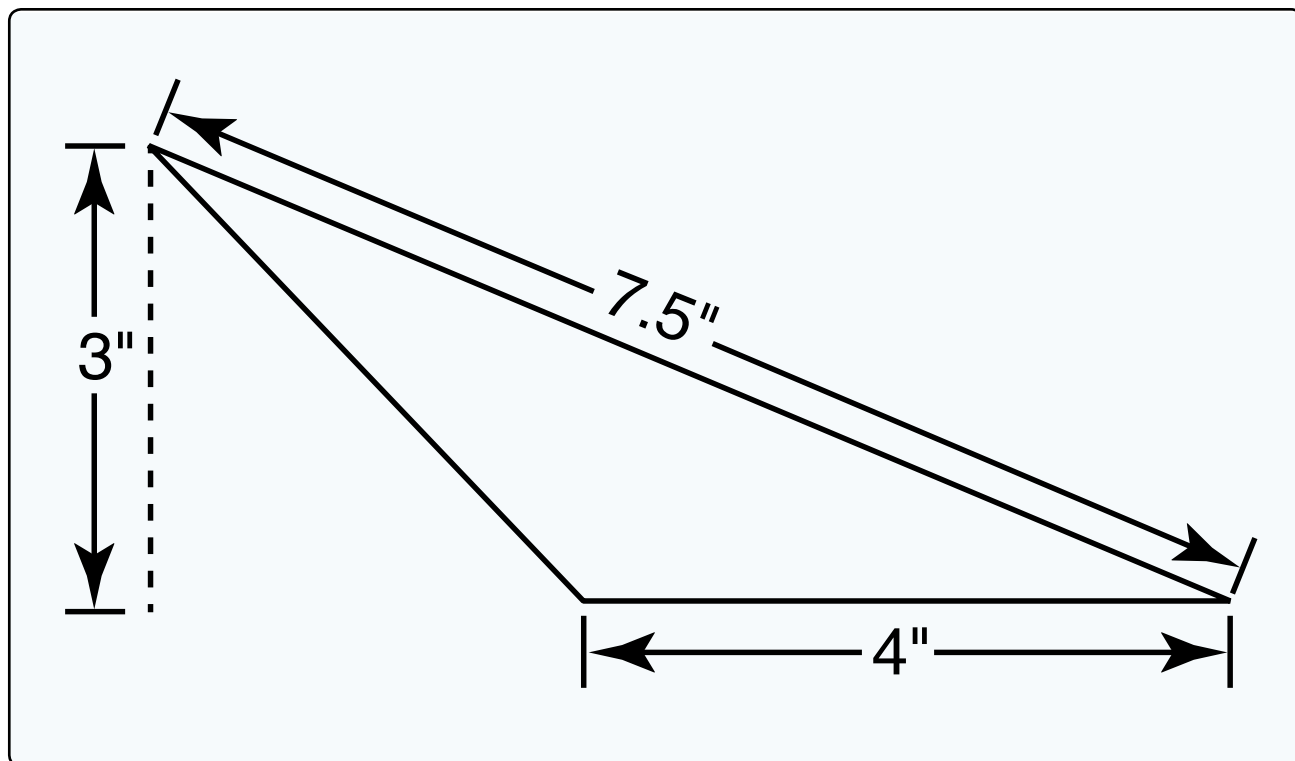
Figure 55. Triangle area.
