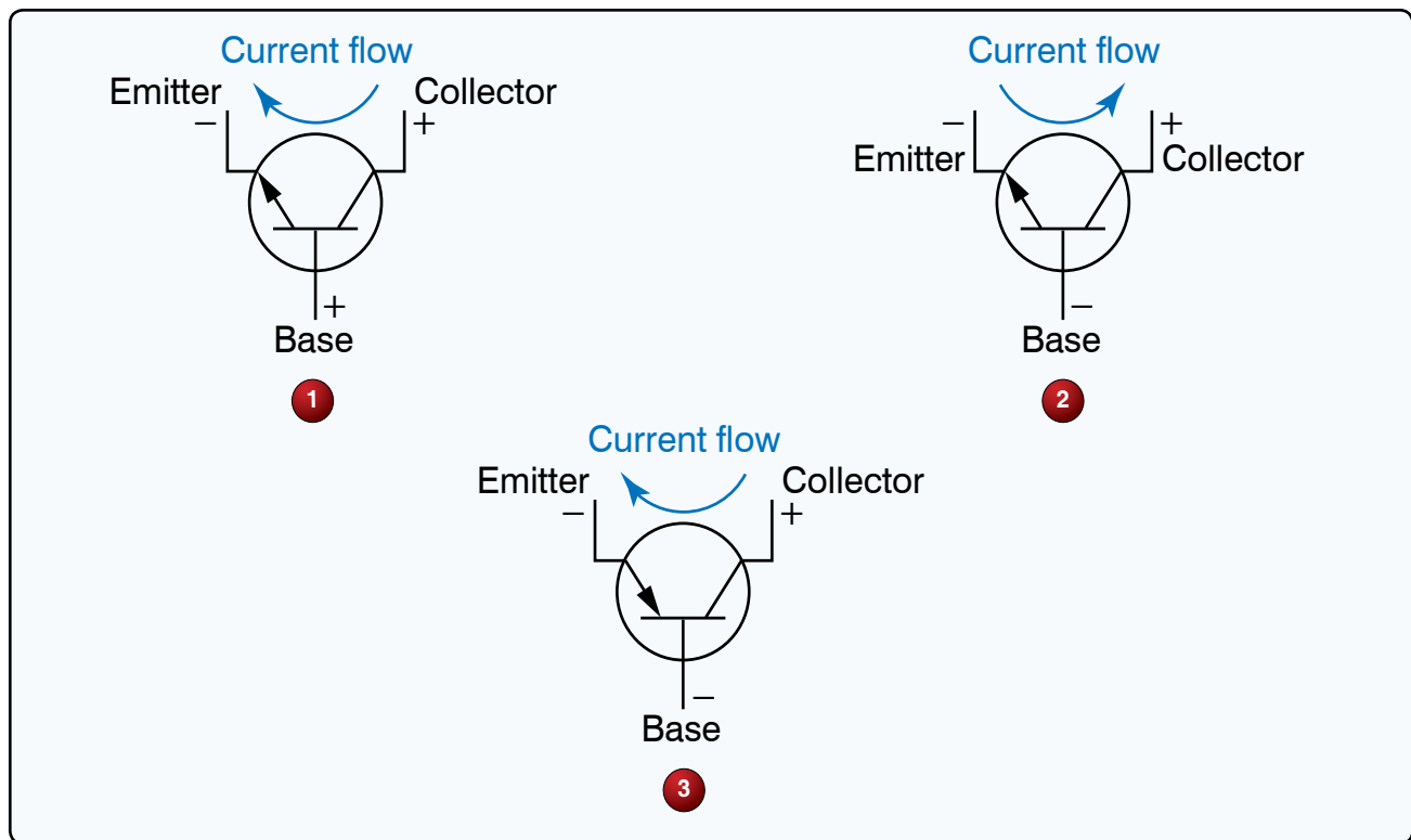
Figure 22. Transistors.
