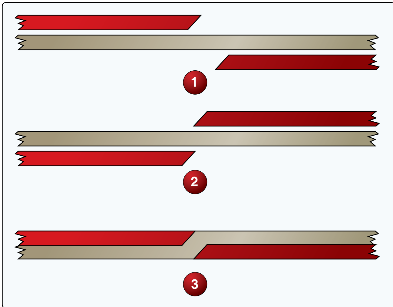
Figure 12. Backup rings.
