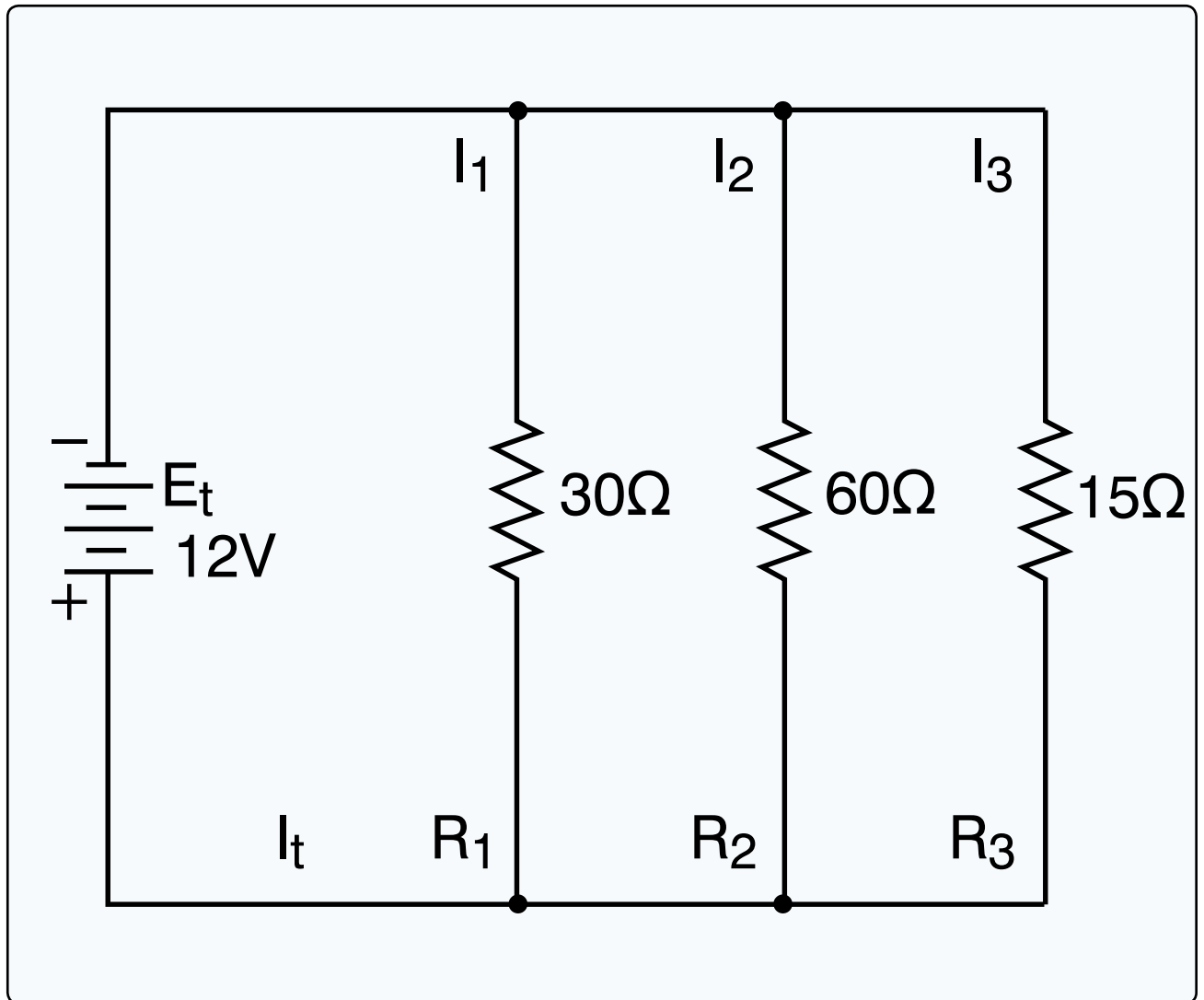
Figure 13. Circuit diagram.
