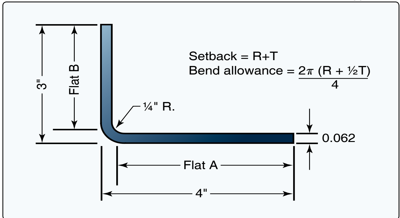
Figure 5. Sheet metal layout.
