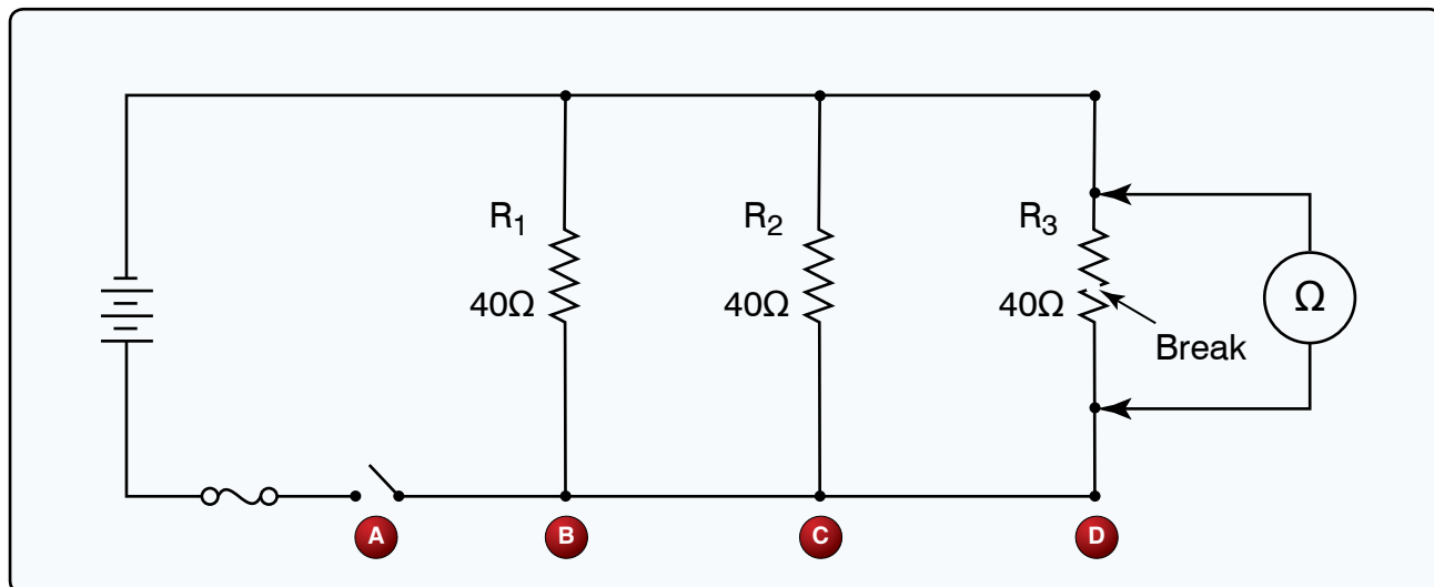
Figure 7. Circuit diagram.
