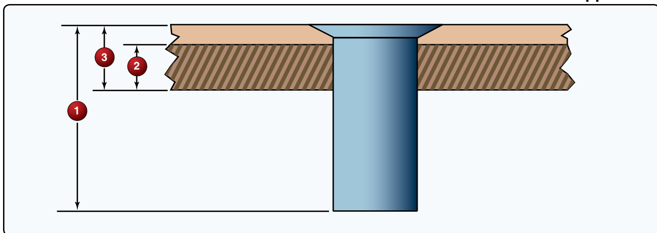
Figure 3. Grip length.
