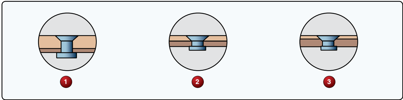
Figure 2. Countersinking.
