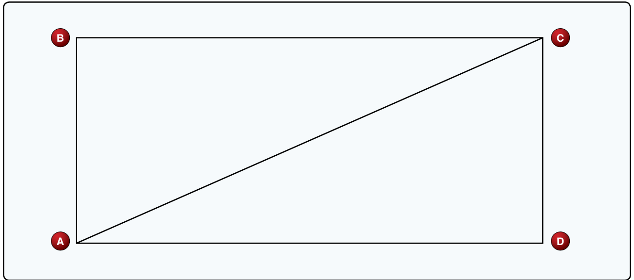
Figure 57. Triangle area.
