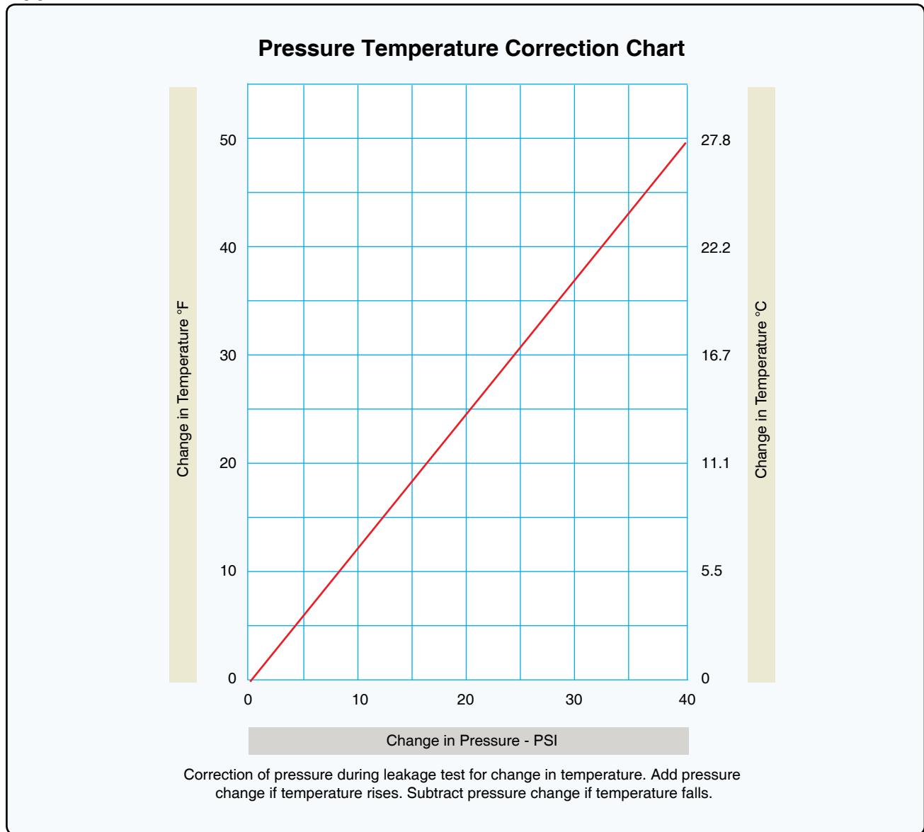
Figure 14. Pressure temperature correction chart.
