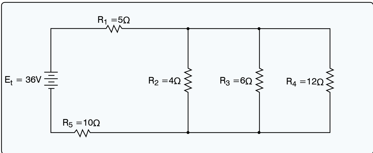
Figure 14. Circuit diagram.
