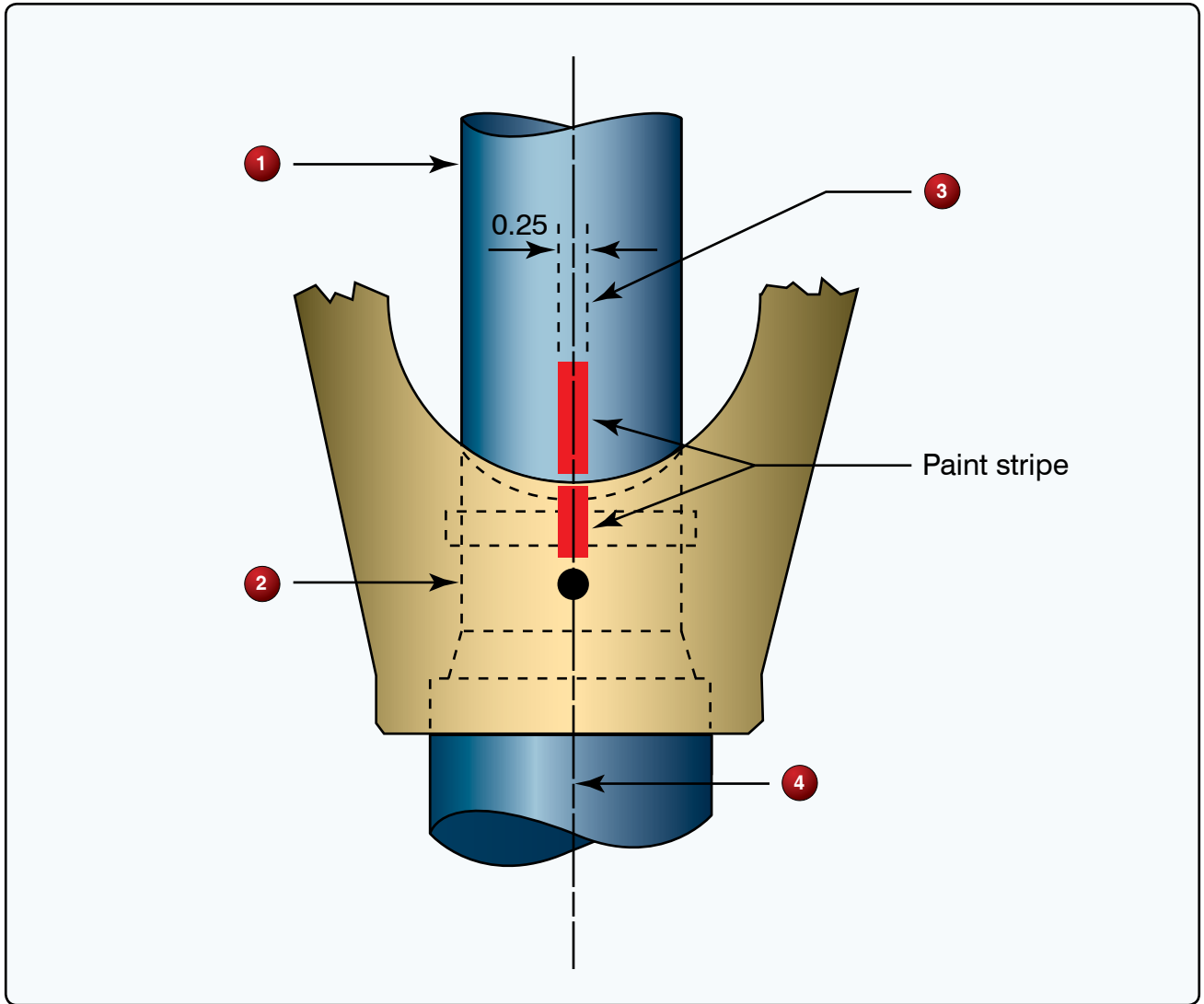
Figure 35. Aircraft drawing.
