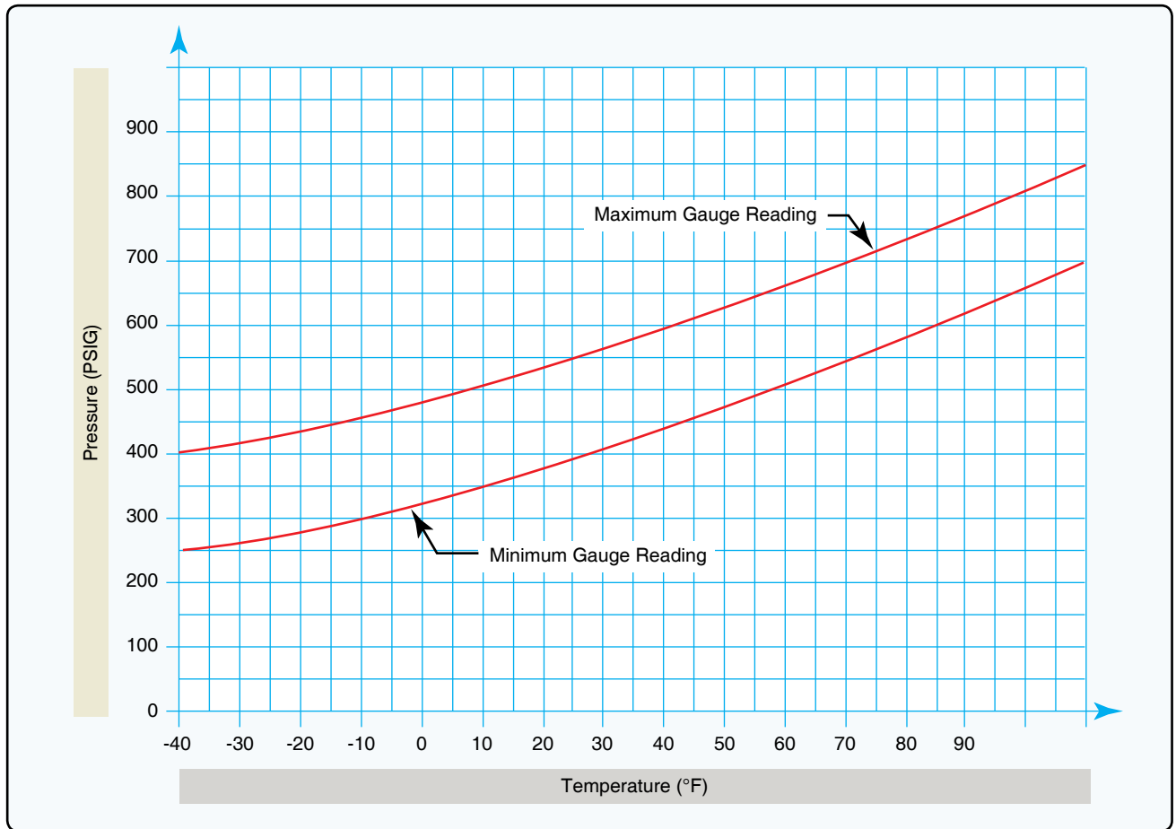
Figure 3. Fire extinguisher pressure chart.
