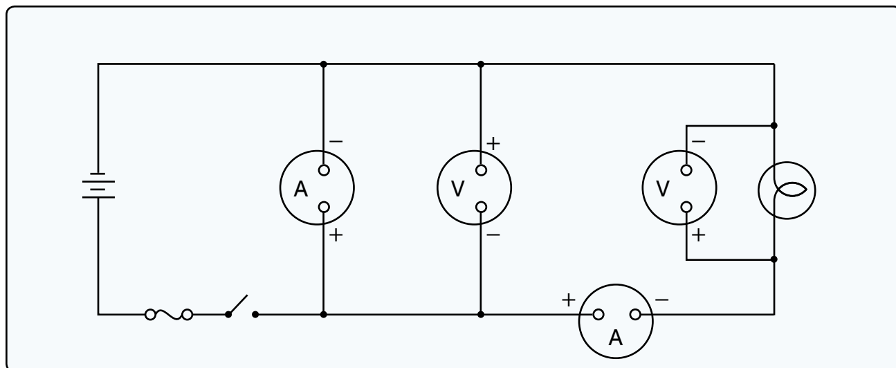
Figure 9. Circuit diagram.
