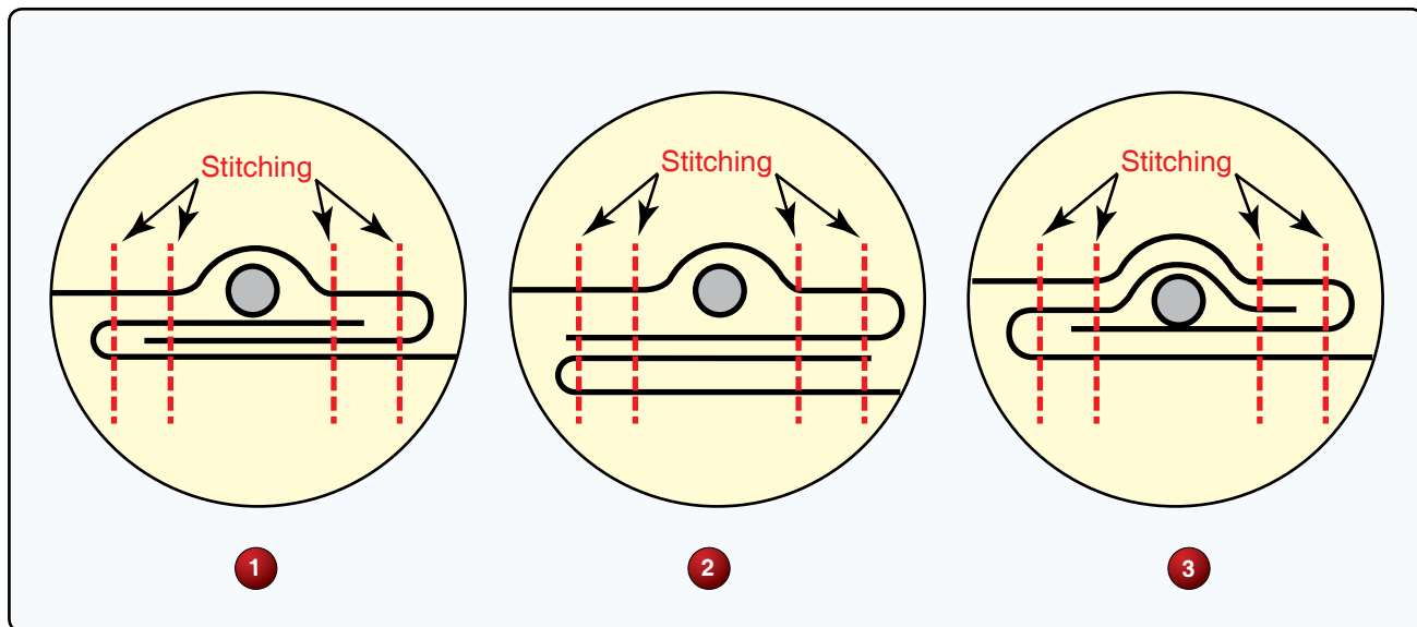
Figure 7. Radial seam stitching.
