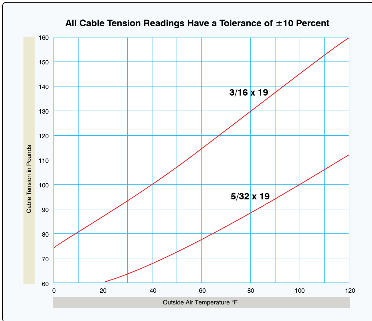
Figure 9. Cable tension chart.
