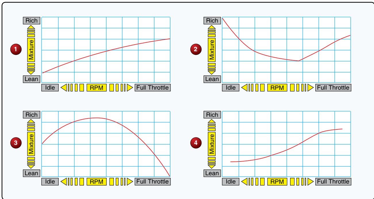
Figure 6. Fuel/air ratio graphs.
