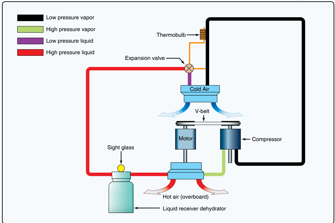
Figure 13. Cooling system.
