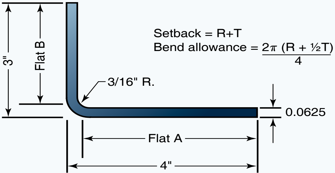
Figure 4. Bending sheet metal.
