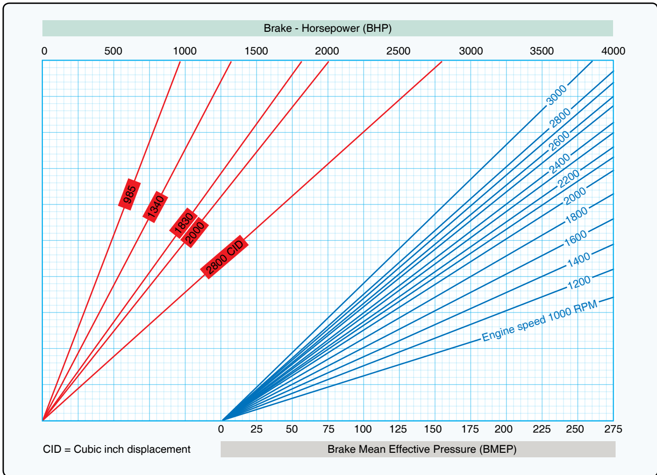
Figure 38. Performance chart.
