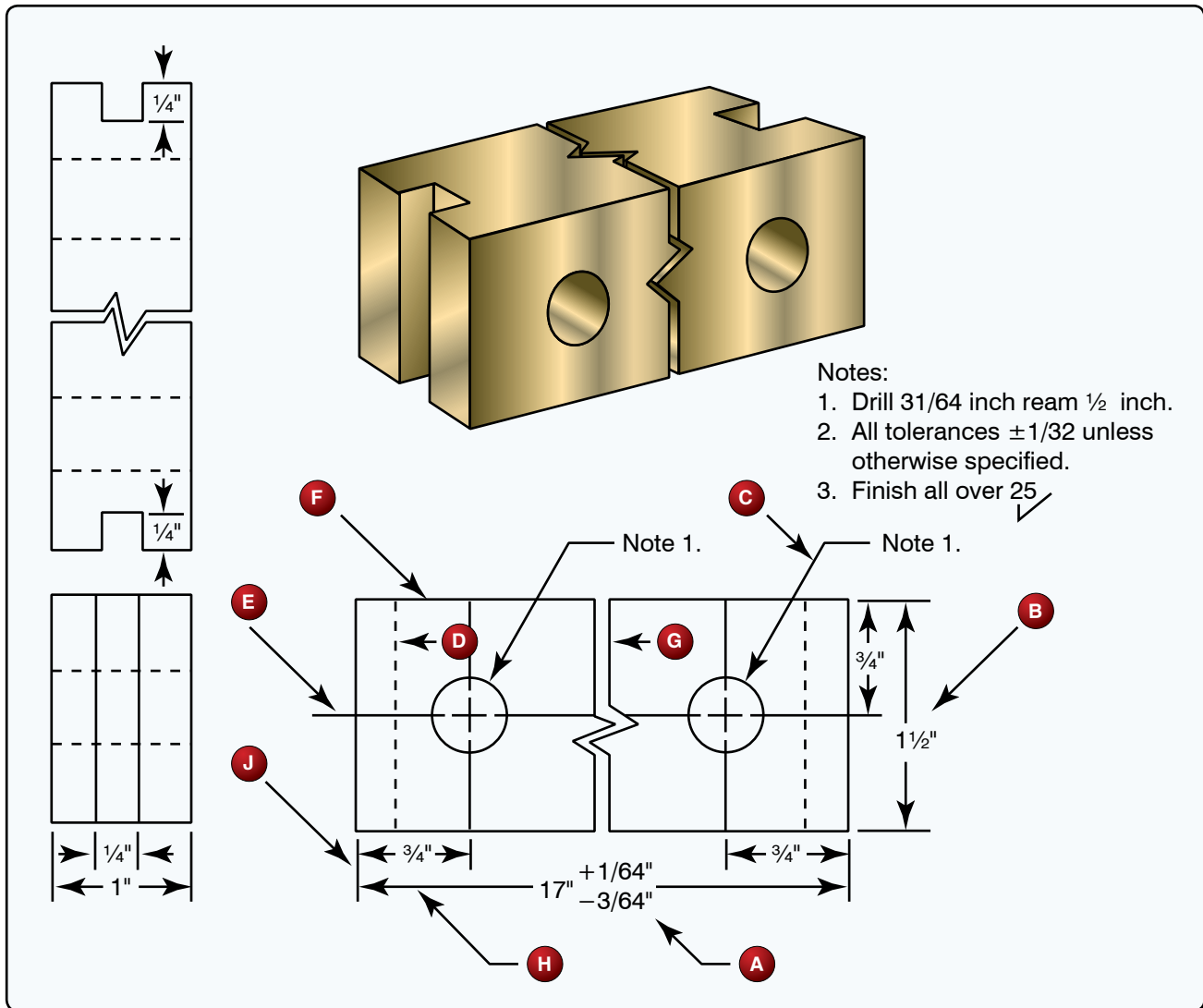
Figure 36. Aircraft drawing.
