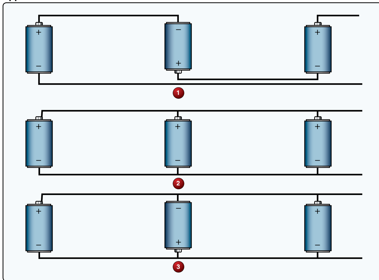
Figure 18. Battery connections.
