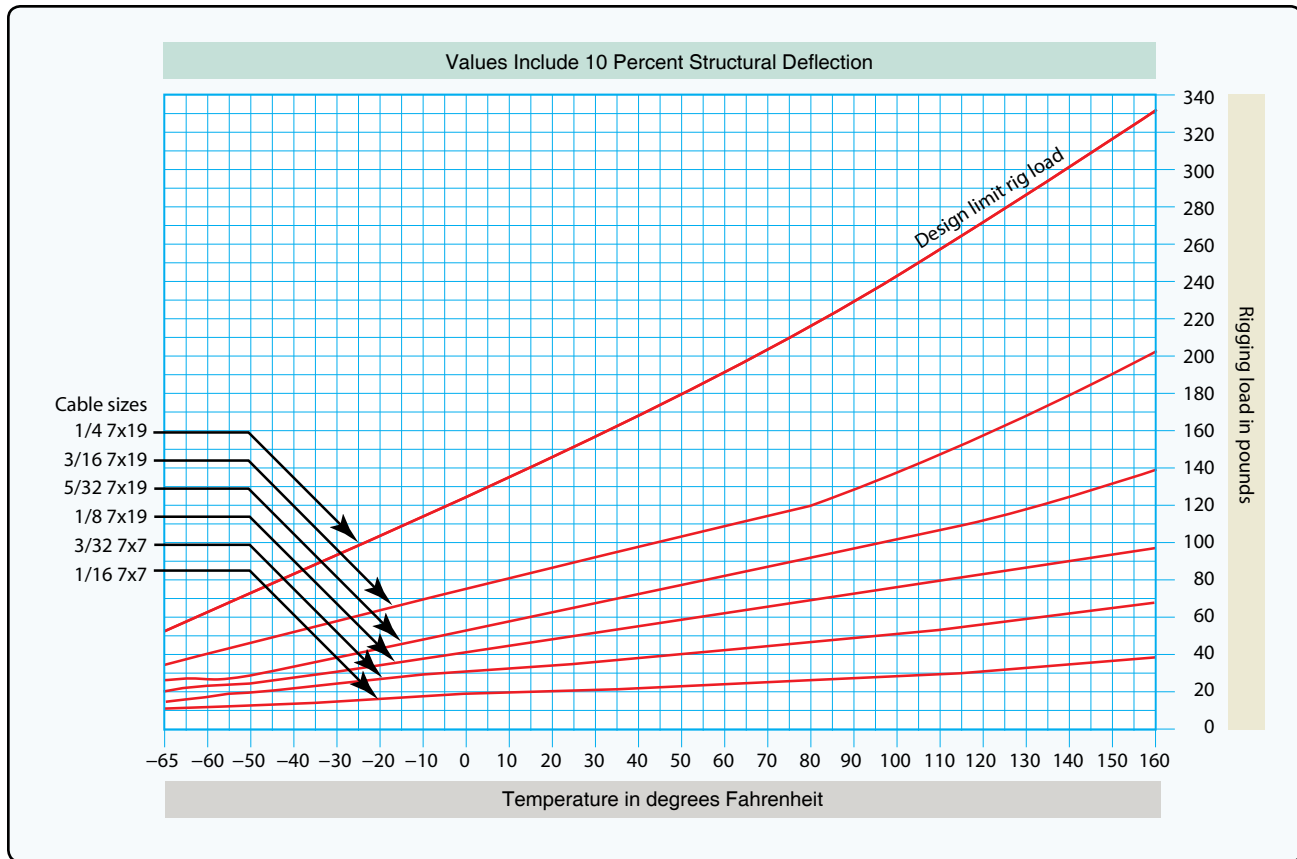
Figure 40. Cable tension chart.
