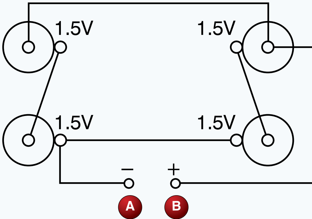
Figure 10. Battery circuit.
