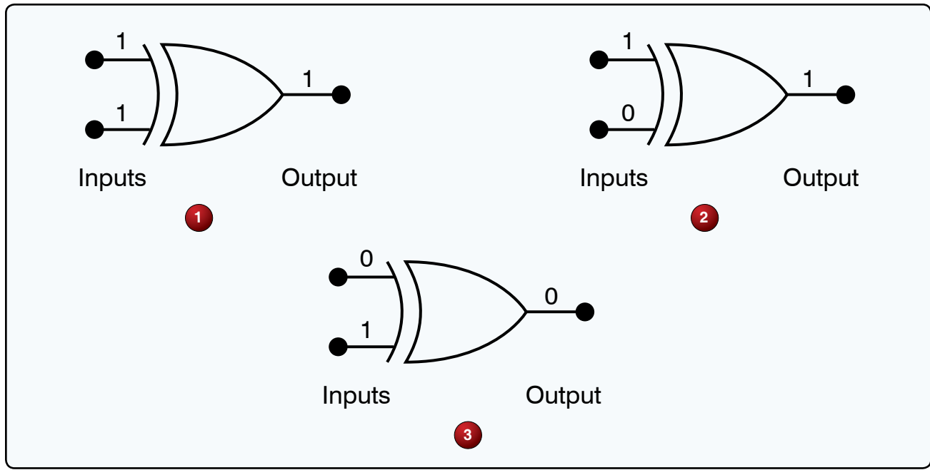
Figure 26. Logic gate.
