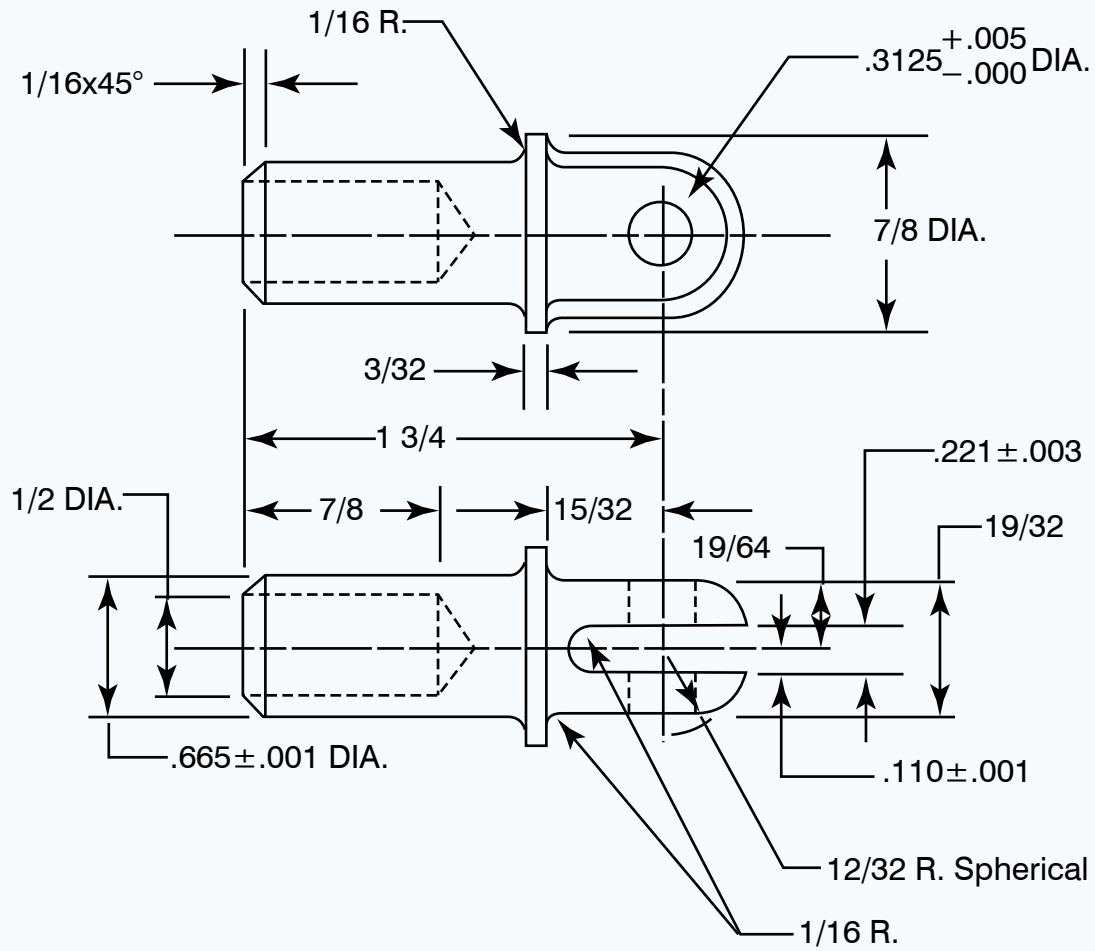
Figure 34. Aircraft drawing.
