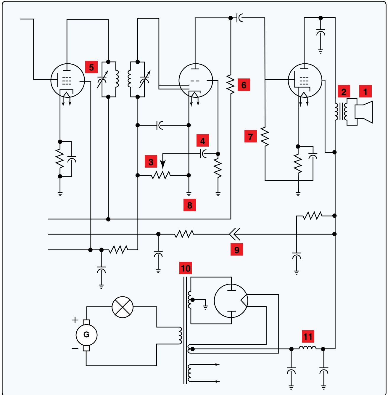
Figure 17. Electrical symbols.
