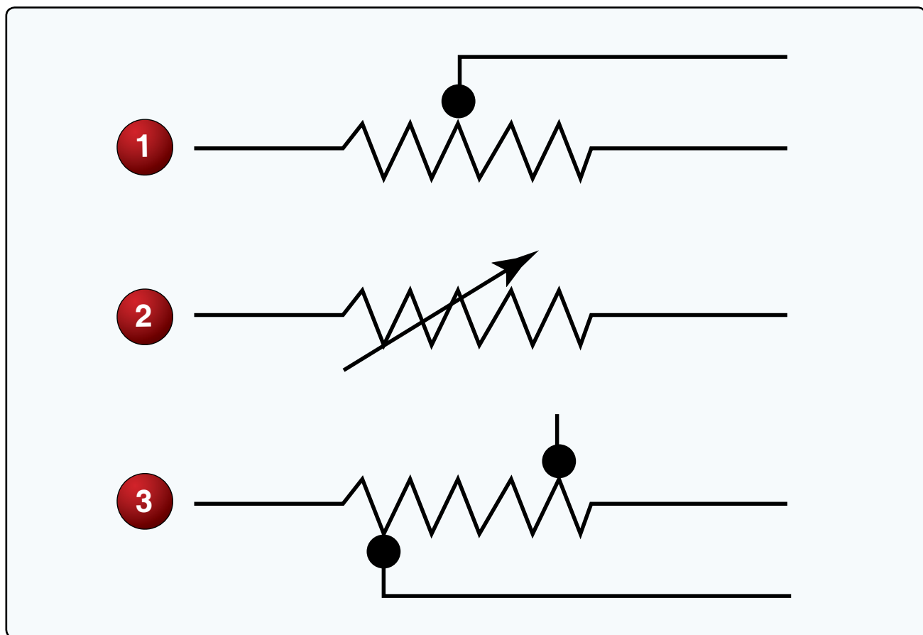
Figure 21. Electrical symbols.
