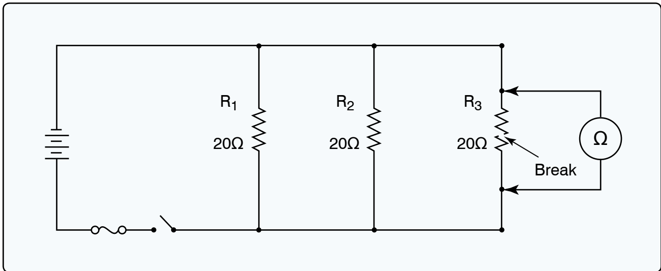
Figure 8. Circuit diagram.
