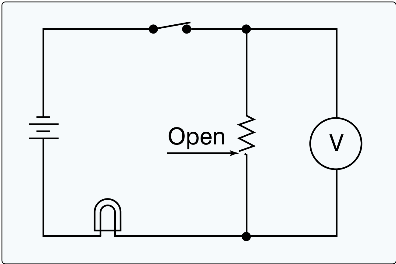
Figure 20. Circuit diagram.
