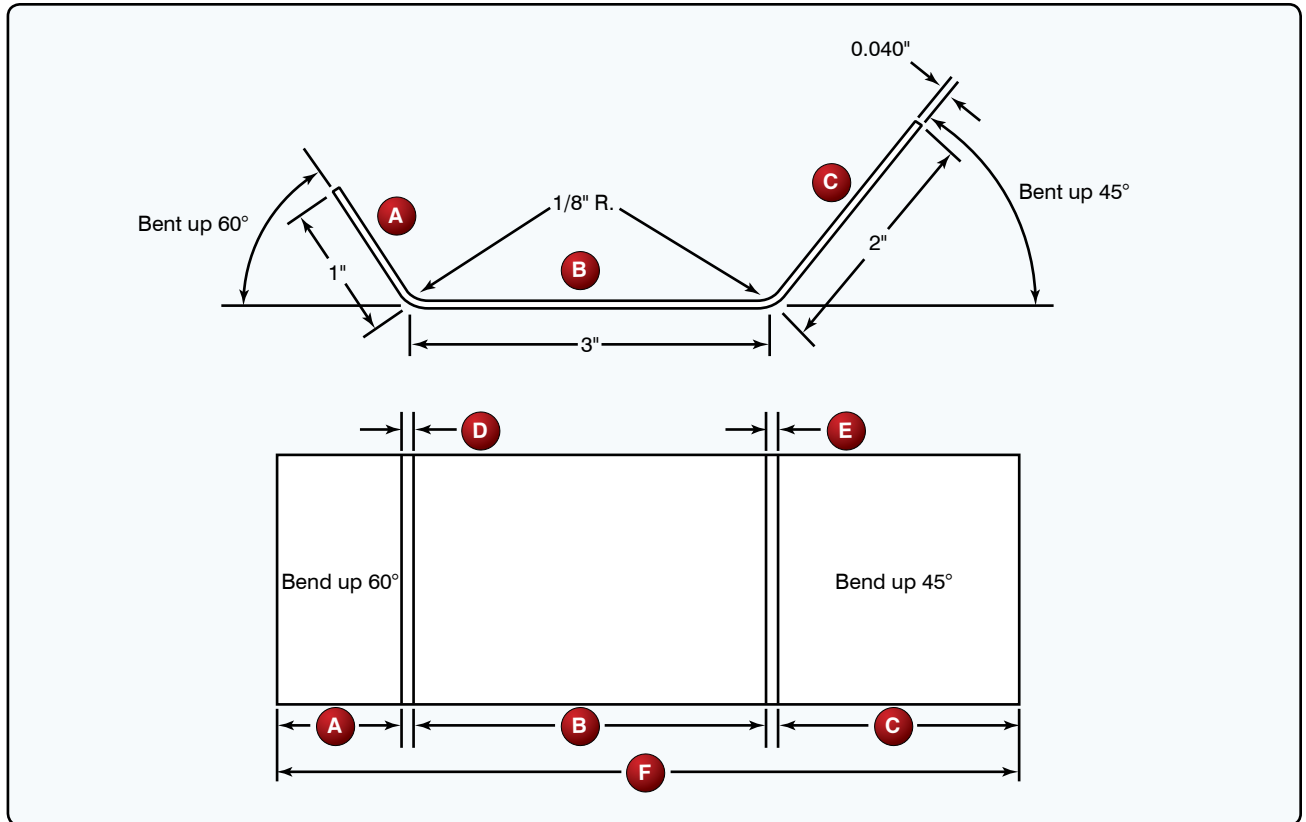
Figure 7. Sheet metal layout.
