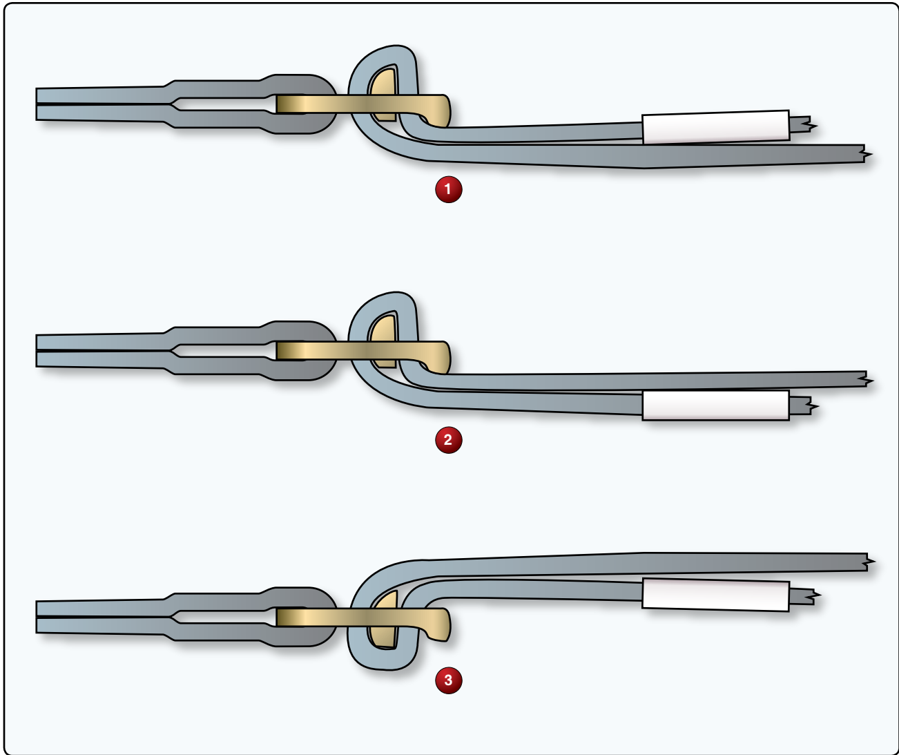
Figure 16. Hardware threading.
