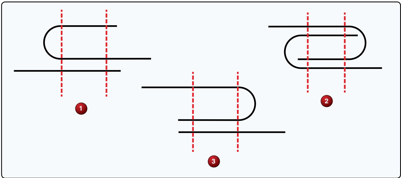
Figure 12. English fell seam.
