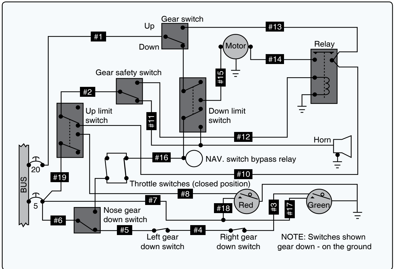
Figure 19. Landing gear circuit.
