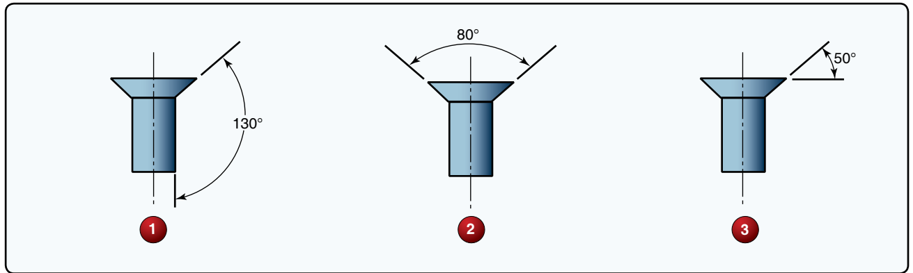
Figure 1. Rivets.
