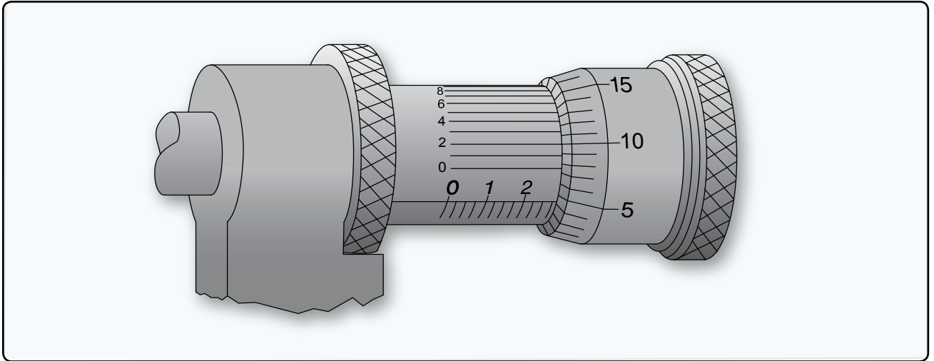
Figure 49. Precision measurement.
