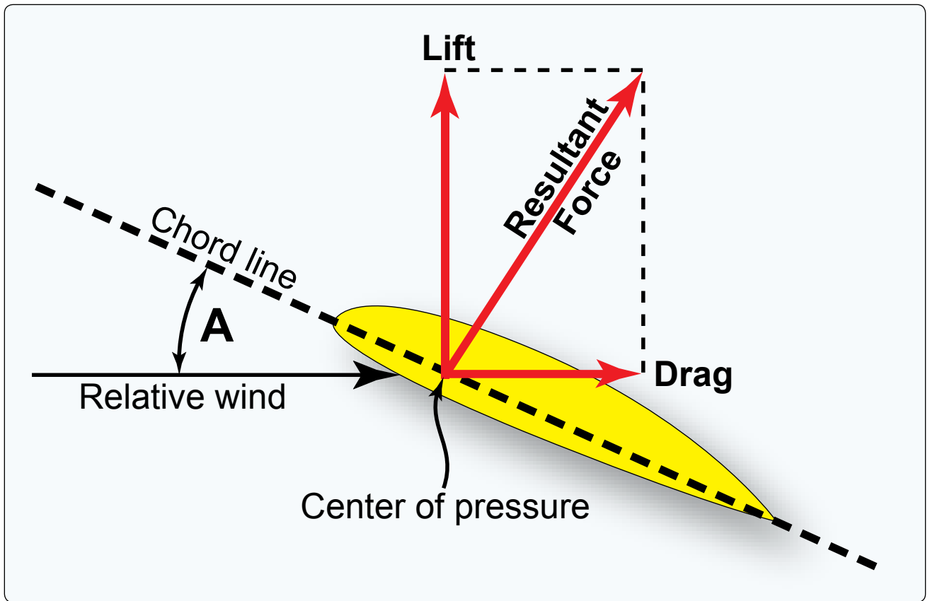
Figure 1. Lift Vector.
