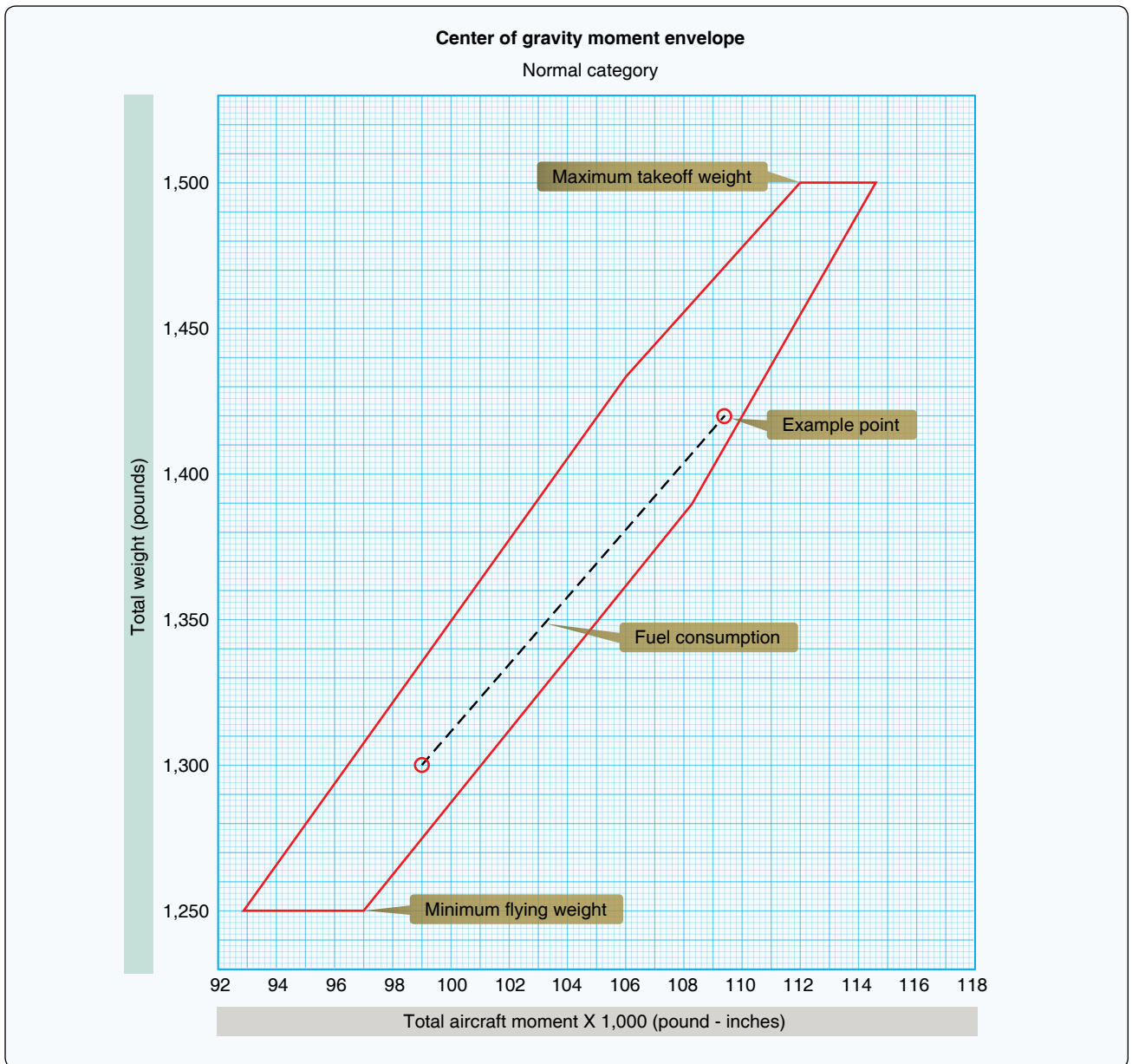
Figure 44. Gyroplane Weight and Balance Graph.
